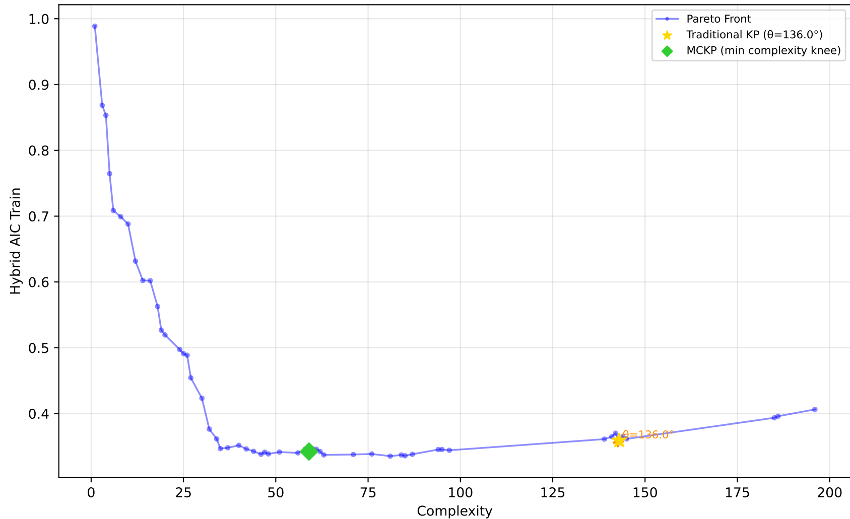
605_fri_c2_250_25 - Run 15 - MVP - Hybrid AIC Train \lambda_1=0.30, \lambda_2=0.00, \lambda_3=1.00 | Difficulty: 1.00 | Method: hmr
