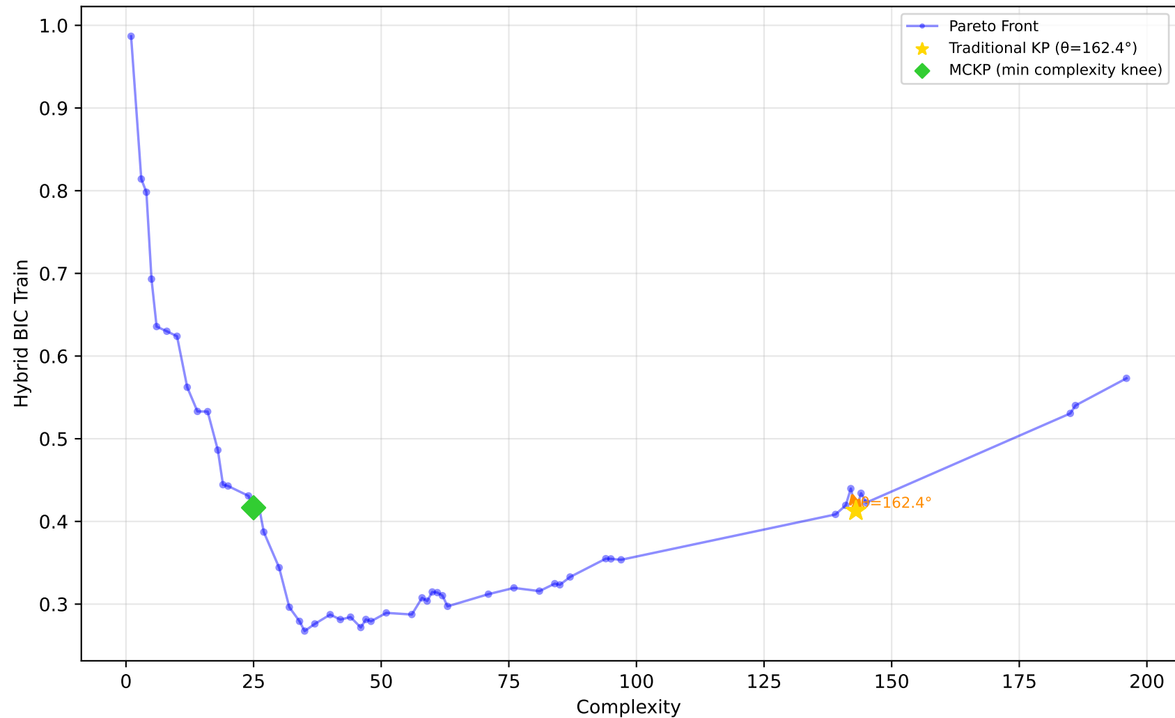
605_fri_c2_250_25 - Run 15 - MVP - Hybrid BIC Train \lambda_1=0.10, \lambda_2=0.00, \lambda_3=0.00 | Difficulty: 1.00 | Method: hmr
