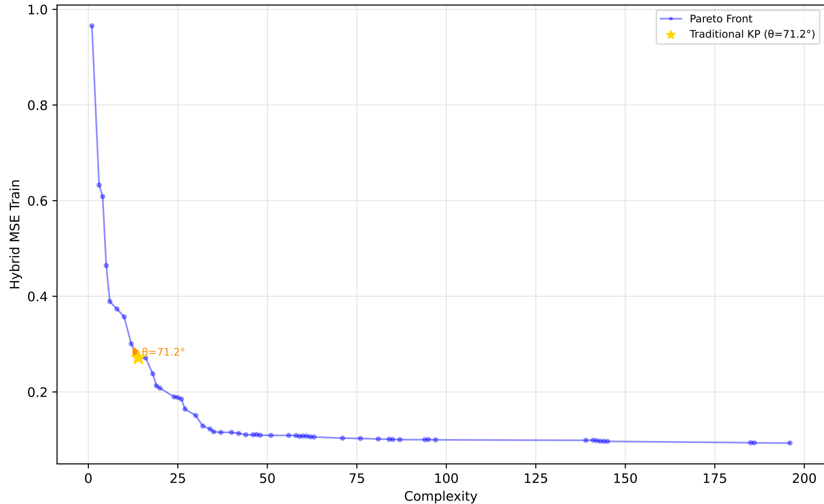
605_fri_c2_250_25 - Run 15 - MVP - Hybrid MSE Train \lambda_1=0.30, \bar{\lambda}_2=0.00, \lambda_3=1.00 | Difficulty: 1.00 | Method: hmr
