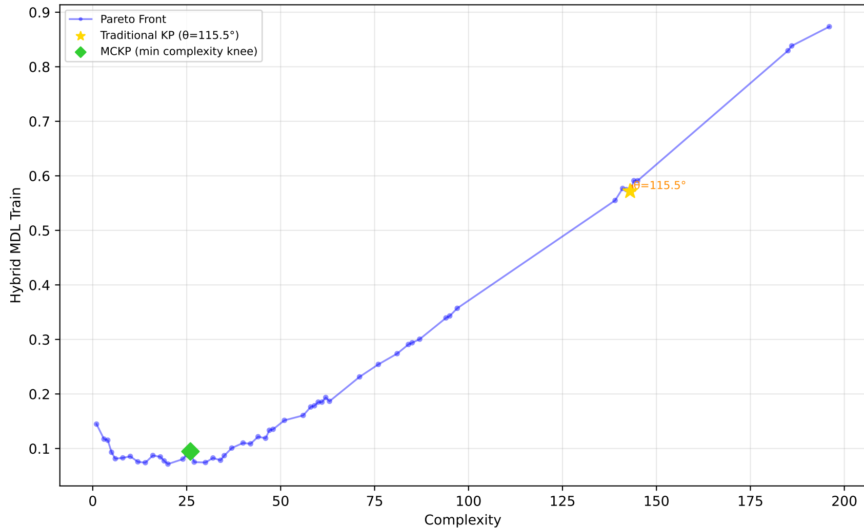
605_fri_c2_250_25 - Run 15 - SVP - Hybrid MDL Train \lambda_1=0.10, \bar{\lambda}_2=0.00, \bar{\lambda}_3=0.00 | Difficulty: 1.00 | Method: hmr
