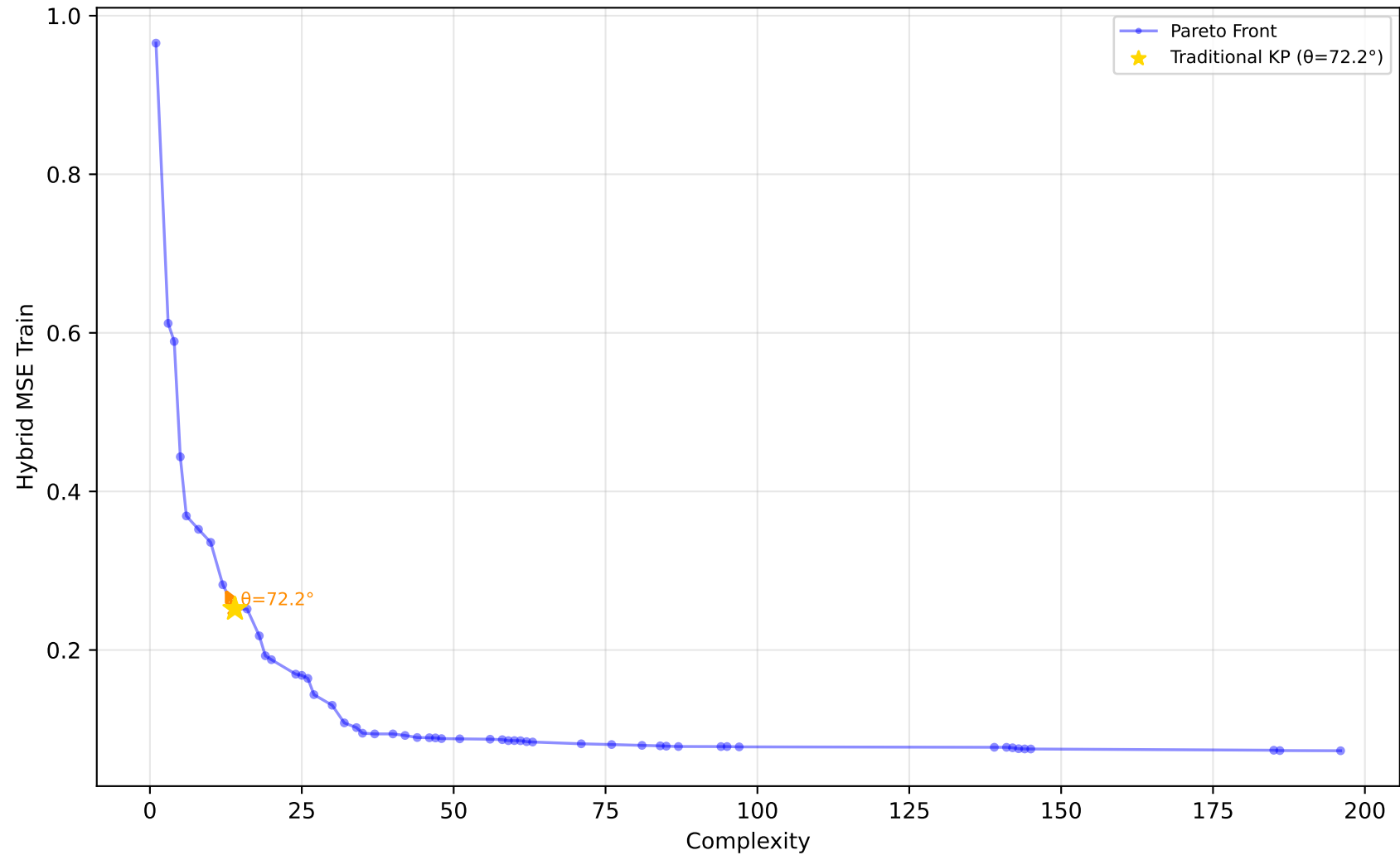
605_fri_c2_250_25 - Run 15 - SVP - Hybrid MSE Train \lambda_1=0.10, \lambda_2=0.00, \lambda_3=0.00 | Difficulty: 1.00 | Method: hmr
