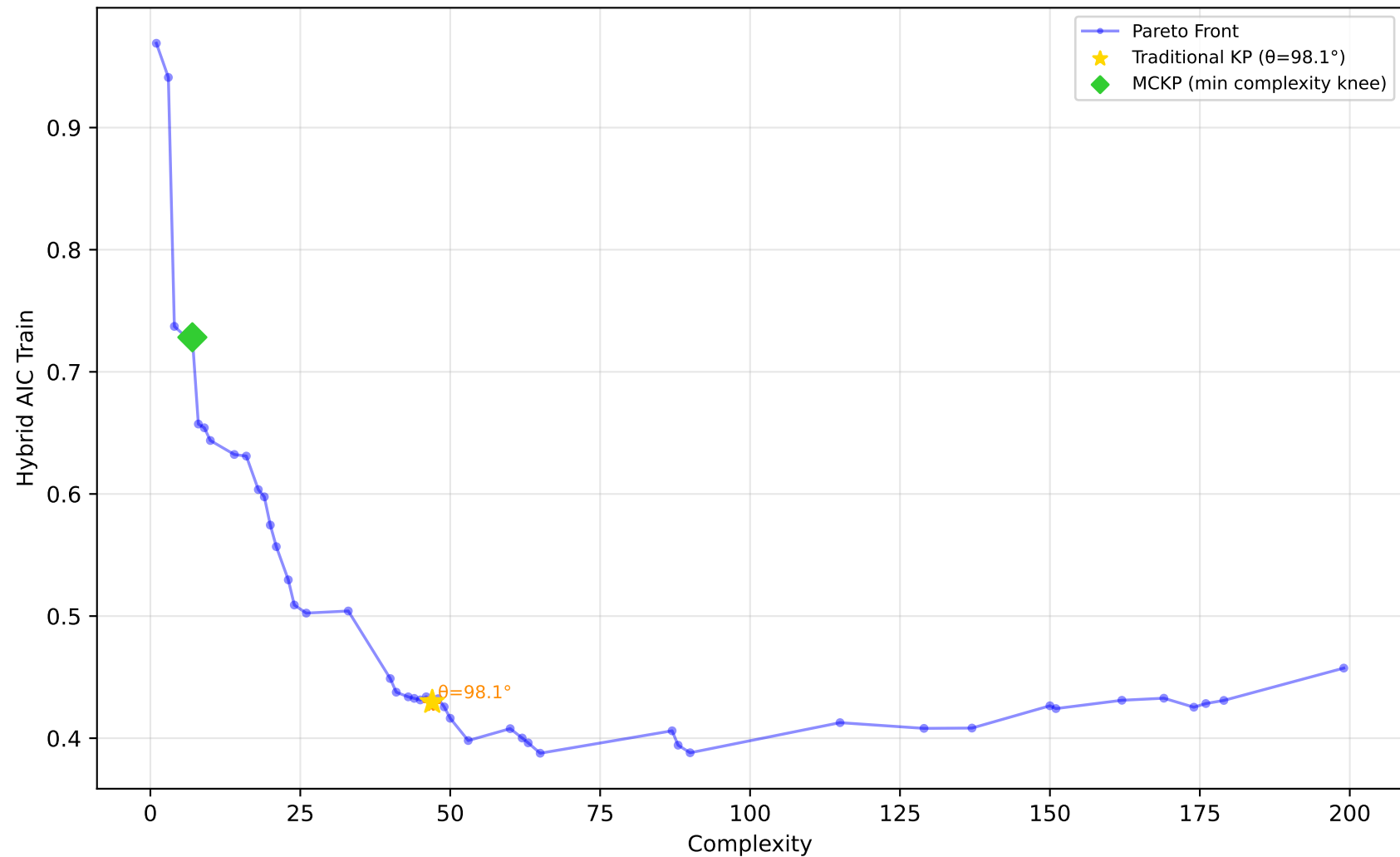
605_fri_c2_250_25 - Run 16 - MVP - Hybrid AIC Train \lambda_1=0.30, \lambda_2=0.00, \lambda_3=1.00 | Difficulty: 1.00 | Method: hmr
