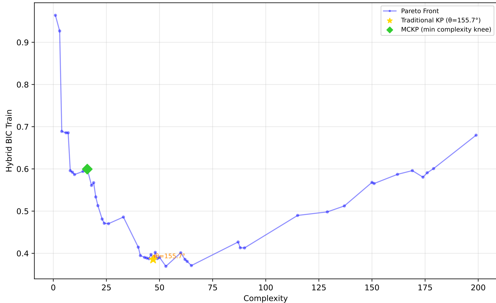
605_fri_c2_250_25 - Run 16 - MVP - Hybrid BIC Train \lambda_1=0.30, \lambda_2=0.00, \lambda_3=1.00 | Difficulty: 1.00 | Method: hmr
