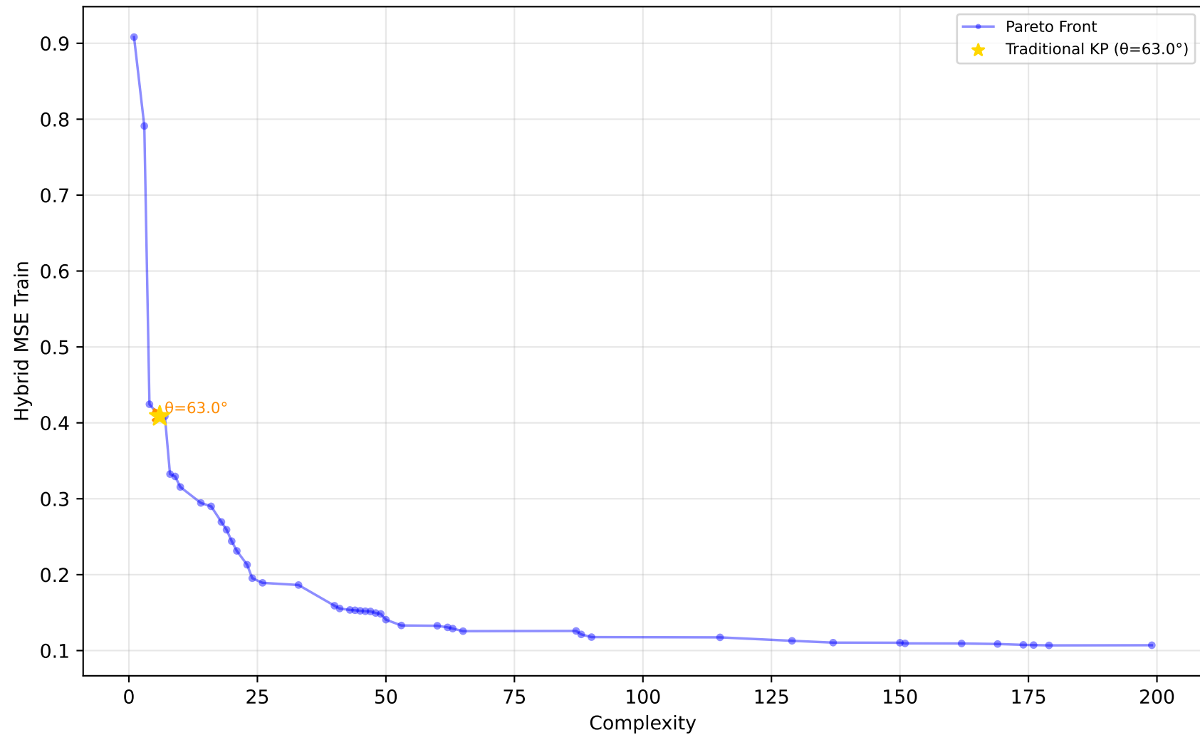
605_fri_c2_250_25 - Run 16 - MVP - Hybrid MSE Train \lambda_1=0.30, \bar{\lambda}_2=0.00, \bar{\lambda}_3=1.00 | Difficulty: 1.00 | Method: hmr
