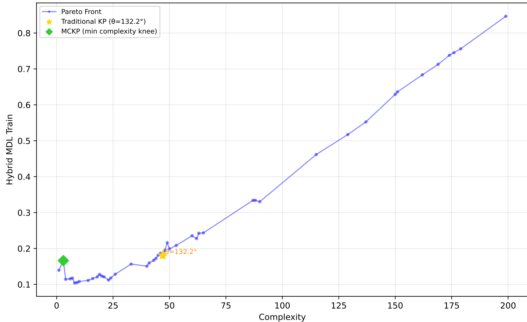
605_fri_c2_250_25 - Run 16 - SVP - Hybrid MDL Train \lambda_1=0.40, \lambda_2=0.00, \lambda_3=0.20 | Difficulty: 1.00 | Method: hmr
