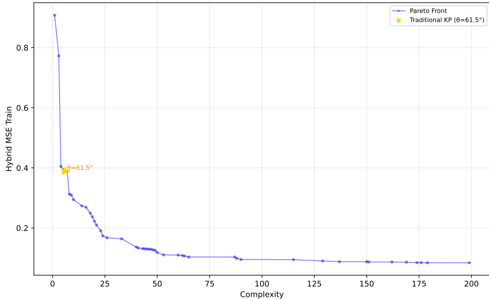
605_fri_c2_250_25 - Run 16 - SVP - Hybrid MSE Train \lambda_1=0.10, \lambda_2=0.00, \lambda_3=0.00 | Difficulty: 1.00 | Method: hmr
