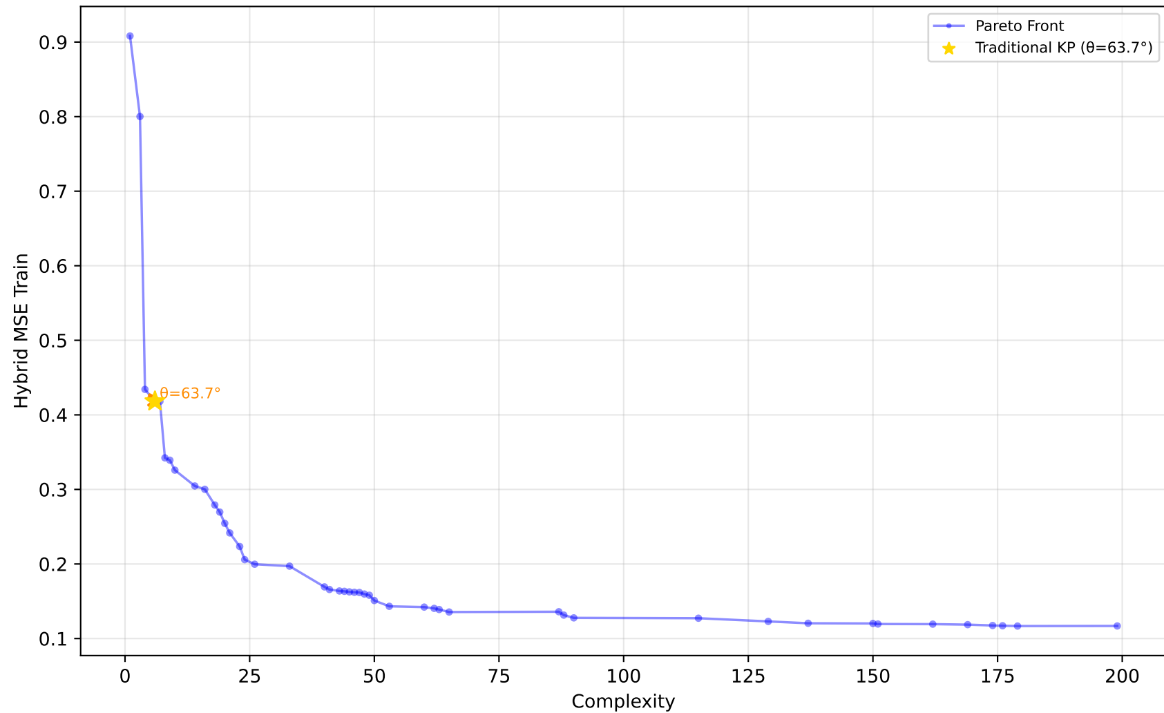
605_fri_c2_250_25 - Run 16 - SVP - Hybrid MSE Train \lambda_1=0.40, \lambda_2=0.00, \lambda_3=0.20 | Difficulty: 1.00 | Method: hmr
