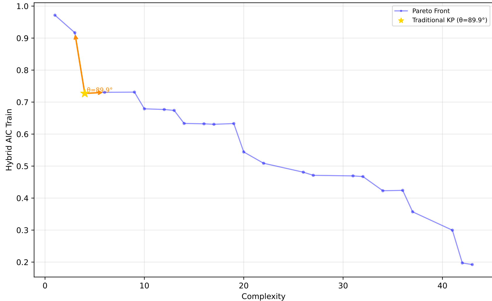
605_fri_c2_250_25 - Run 17 - MVP - Hybrid AIC Train \lambda_1=0.10, \lambda_2=0.00, \lambda_3=0.00 | Difficulty: 1.00 | Method: hmr
