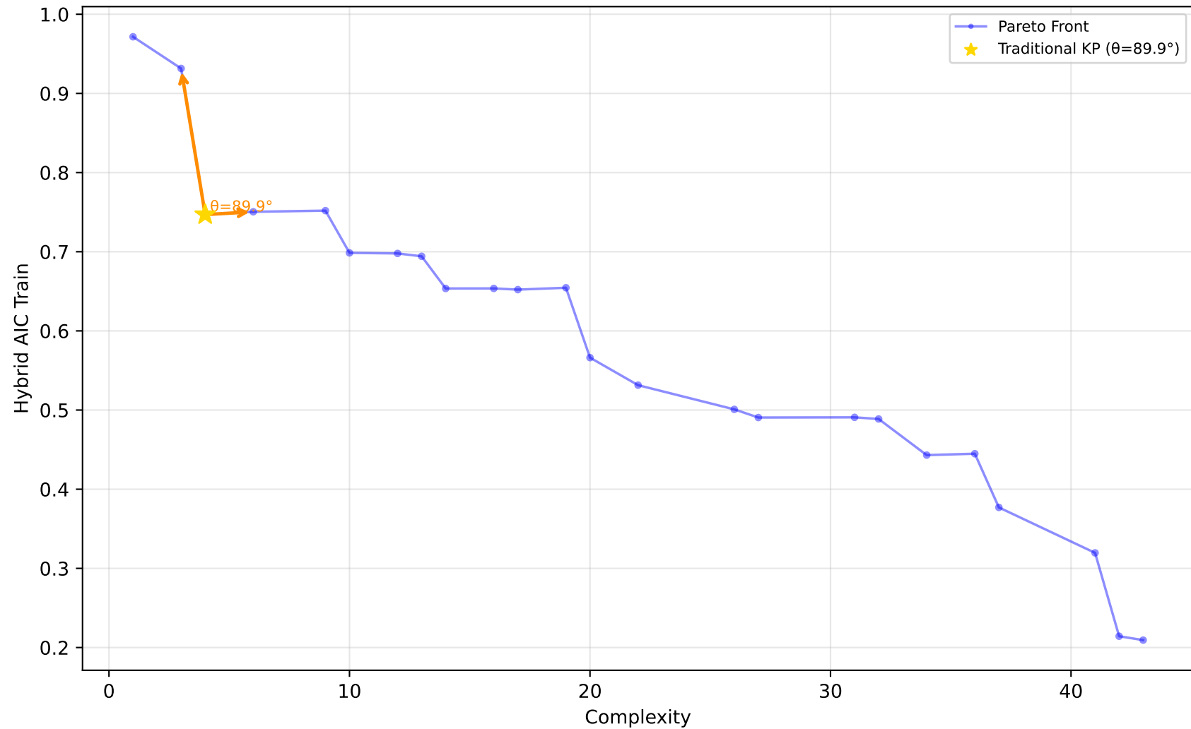
605_fri_c2_250_25 - Run 17 - MVP - Hybrid AIC Train \lambda_1=0.30, \lambda_2=0.00, \lambda_3=1.00 | Difficulty: 1.00 | Method: hmr
