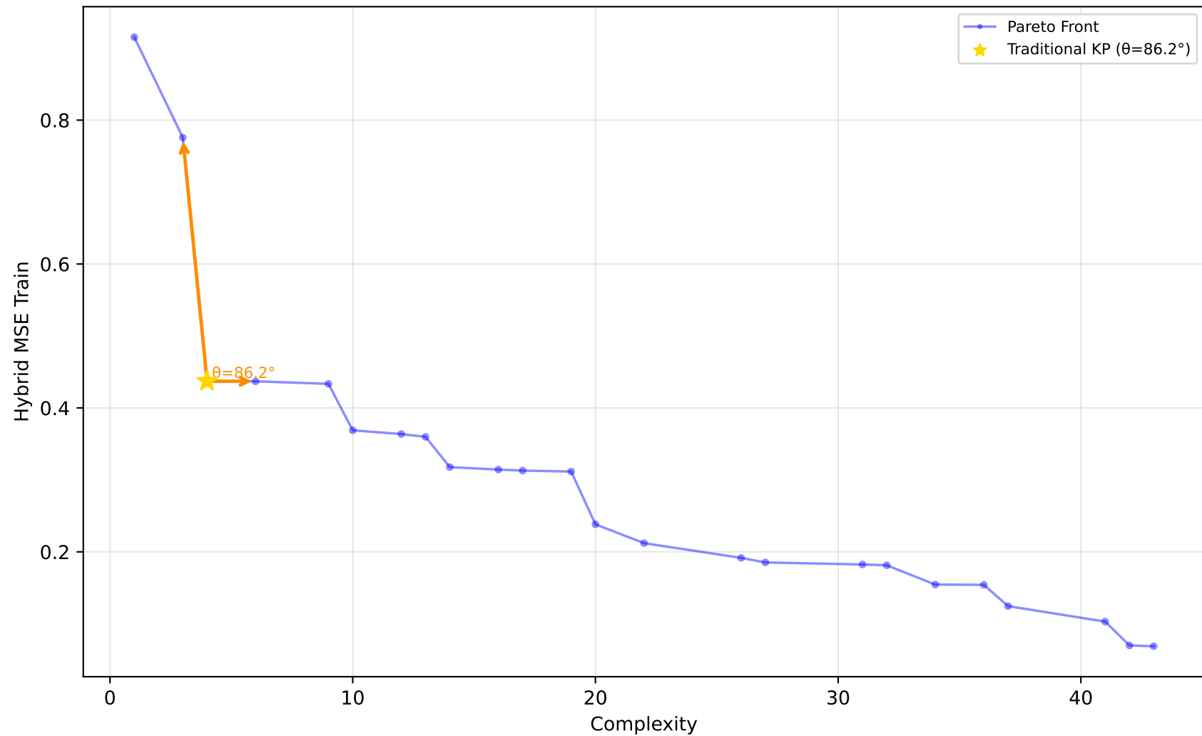
605_fri_c2_250_25 - Run 17 - MVP - Hybrid MSE Train \lambda_1=0.30, \bar{\lambda}_2=0.00, \bar{\lambda}_3=1.00 | Difficulty: 1.00 | Method: hmr
