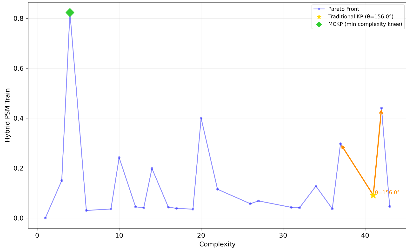
605_fri_c2_250_25 - Run 17 - MVP - Hybrid PSM Train \lambda_1=0.30, \lambda_2=0.00, \lambda_3=1.00 | Difficulty: 1.00 | Method: hmr
