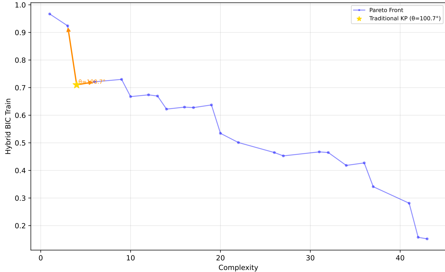
605_fri_c2_250_25 - Run 17 - SVP - Hybrid BIC Train \lambda_1=0.40, \lambda_2=0.00, \lambda_3=0.20 | Difficulty: 1.00 | Method: hmr
