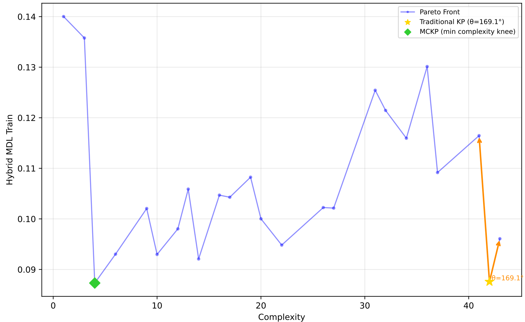
605_fri_c2_250_25 - Run 17 - SVP - Hybrid MDL Train \lambda_1=0.10 , \lambda_2=0.00 , \lambda_3=0.00 | Difficulty: 1.00 | Method: hmr
