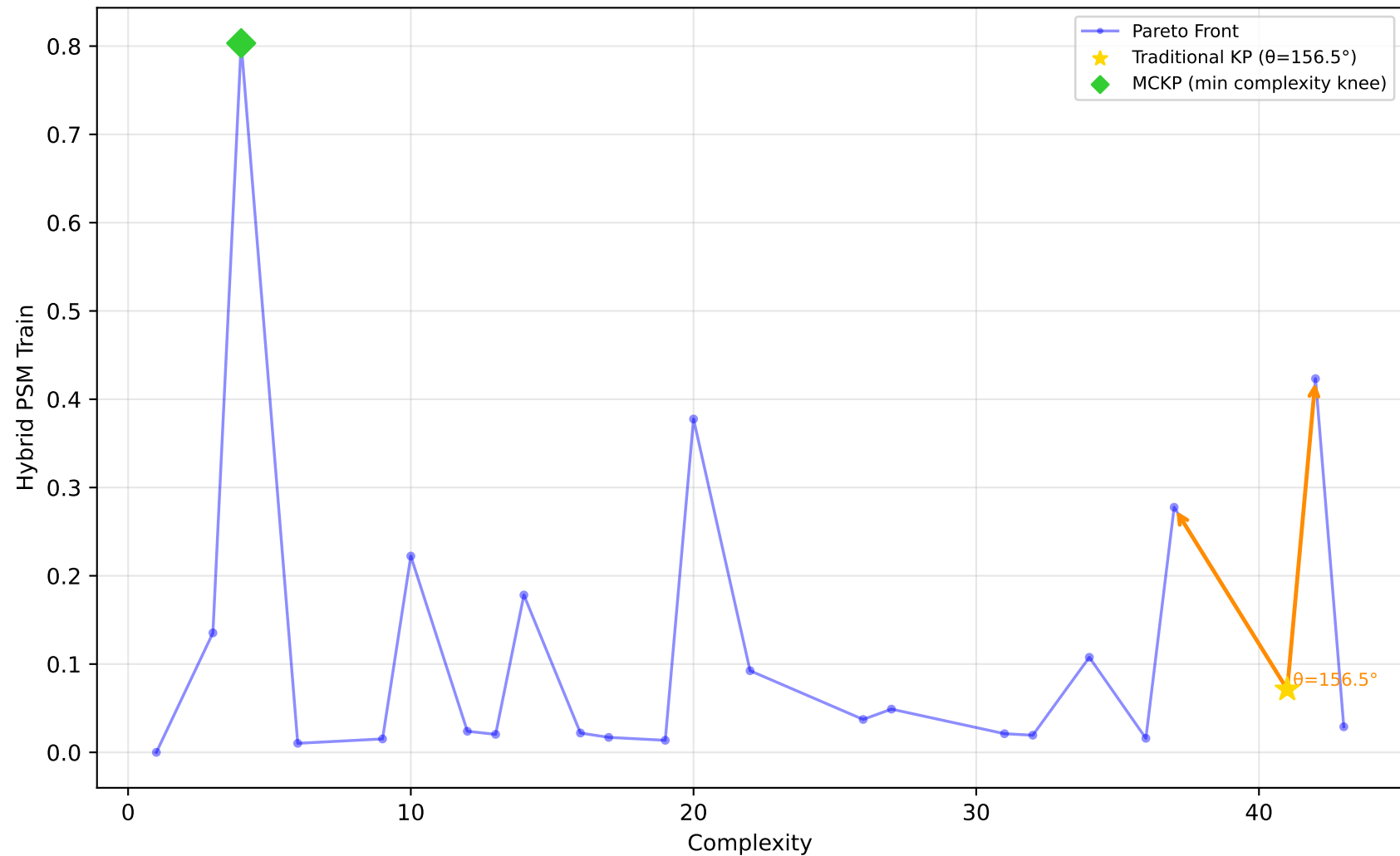
605_fri_c2_250_25 - Run 17 - SVP - Hybrid PSM Train \lambda_1=0.10, \lambda_2=0.00, \lambda_3=0.00 | Difficulty: 1.00 | Method: hmr
