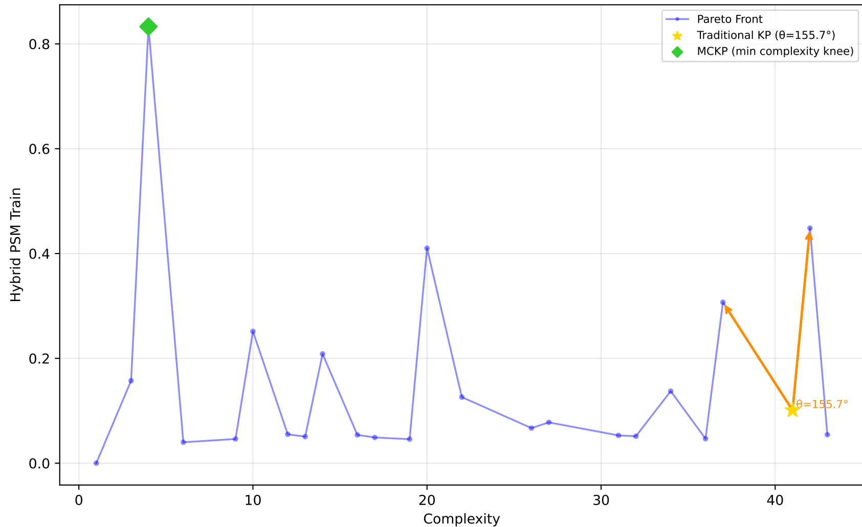
605_fri_c2_250_25 - Run 17 - SVP - Hybrid PSM Train \lambda_1=0.40, \lambda_2=0.00, \lambda_3=0.20 | Difficulty: 1.00 | Method: hmr
