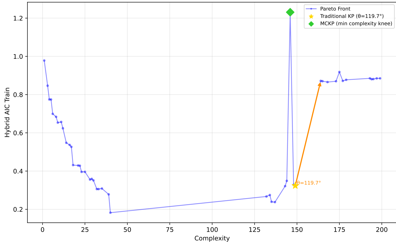
605_fri_c2_250_25 - Run 18 - MVP - Hybrid AIC Train \lambda_1=0.30, \lambda_2=0.00, \lambda_3=1.00 | Difficulty: 1.00 | Method: hmr
