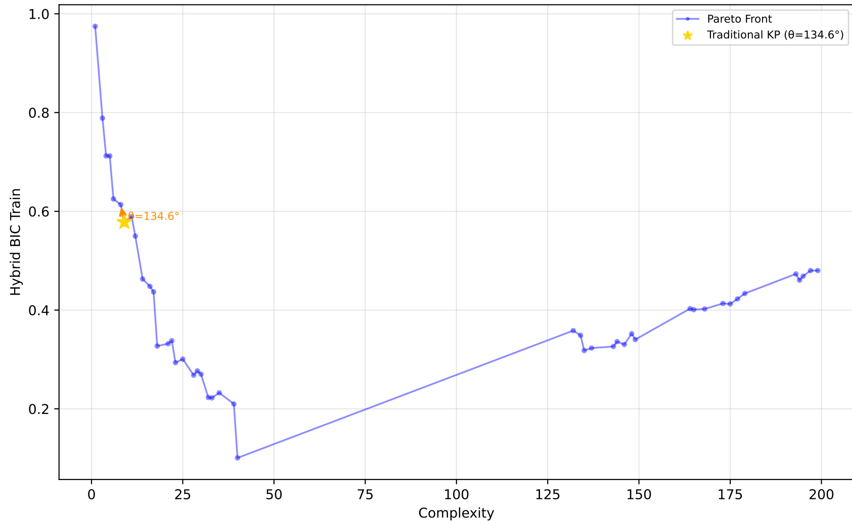
605_fri_c2_250_25 - Run 18 - MVP - Hybrid BIC Train \lambda_1=0.10, \lambda_2=0.00, \lambda_3=0.00 | Difficulty: 1.00 | Method: hmr
