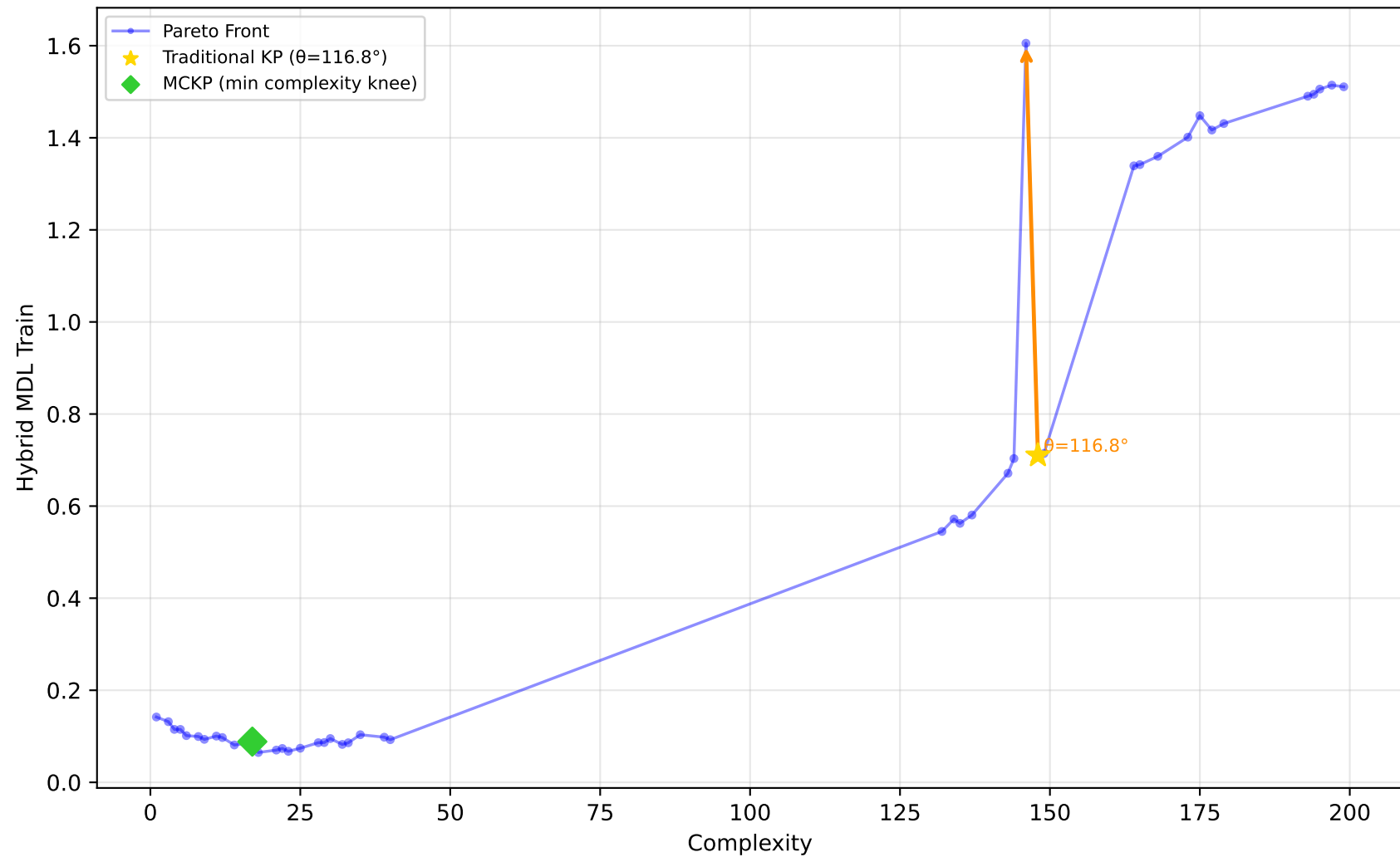
605_fri_c2_250_25 - Run 18 - MVP - Hybrid MDL Train \lambda_1=0.30, \bar{\lambda}_2=0.00, \bar{\lambda}_3=1.00 | Difficulty: 1.00 | Method: hmr
