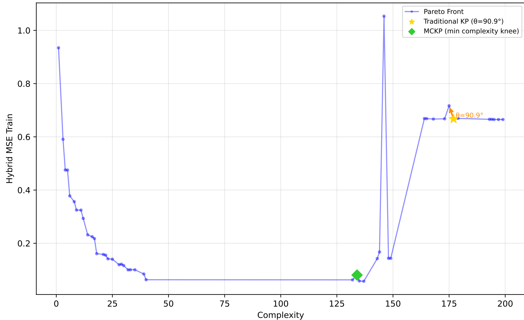
605_fri_c2_250_25 - Run 18 - MVP - Hybrid MSE Train \lambda_1=0.30, \bar{\lambda}_2=0.00, \bar{\lambda}_3=1.00 | Difficulty: 1.00 | Method: hmr
