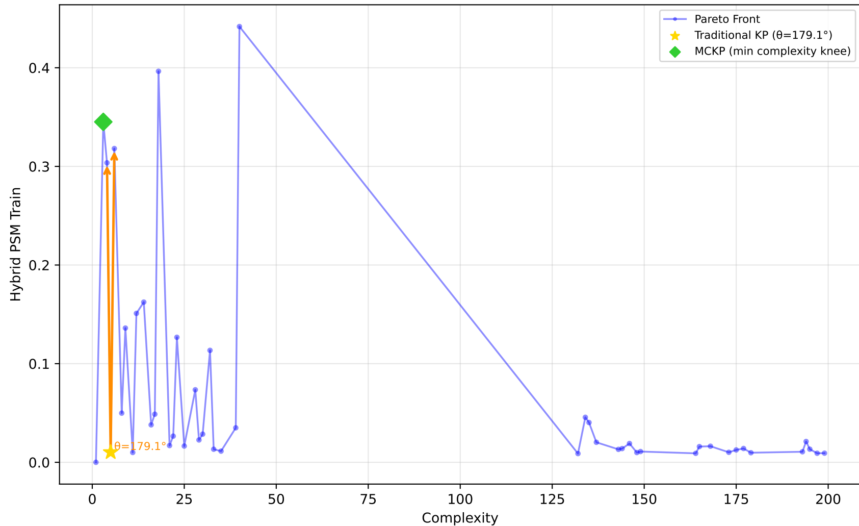
605_fri_c2_250_25 - Run 18 - MVP - Hybrid PSM Train \lambda_1=0.10, \bar{\lambda}_2=0.00, \bar{\lambda}_3=0.00 | Difficulty: 1.00 | Method: hmr
