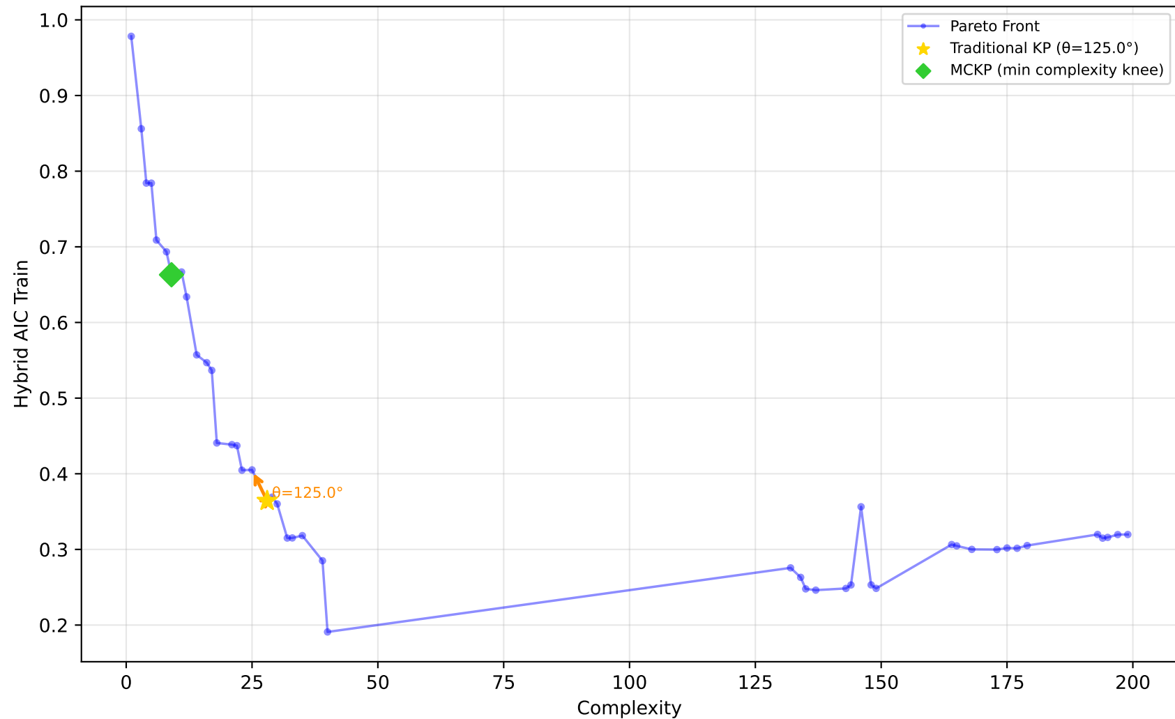
605_fri_c2_250_25 - Run 18 - SVP - Hybrid AIC Train \lambda_1=0.40 , \lambda_2=0.00 , \lambda_3=0.20 | Difficulty: 1.00 | Method: hmr
