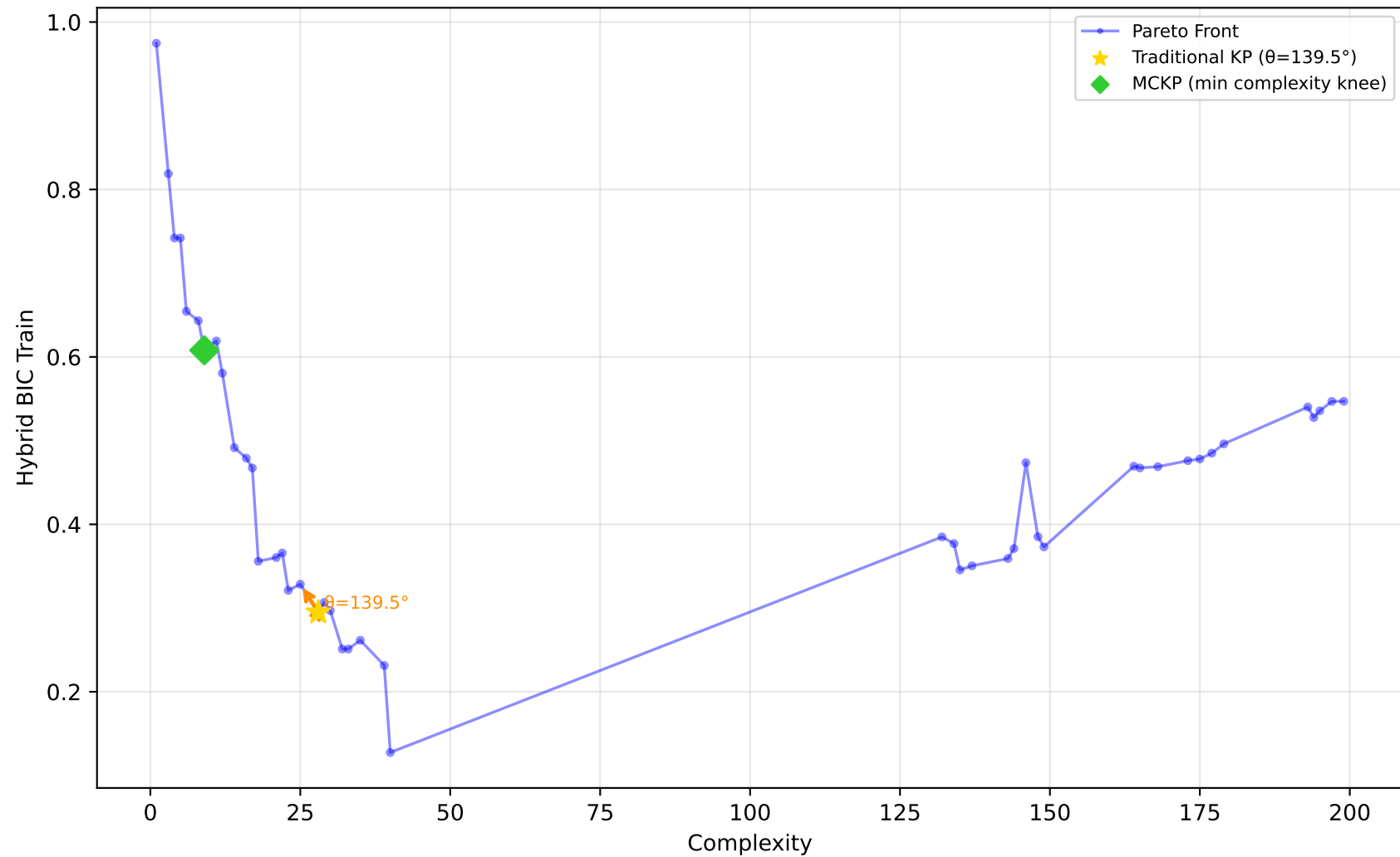
605_fri_c2_250_25 - Run 18 - SVP - Hybrid BIC Train \lambda_1=0.40, \lambda_2=0.00, \lambda_3=0.20 | Difficulty: 1.00 | Method: hmr
