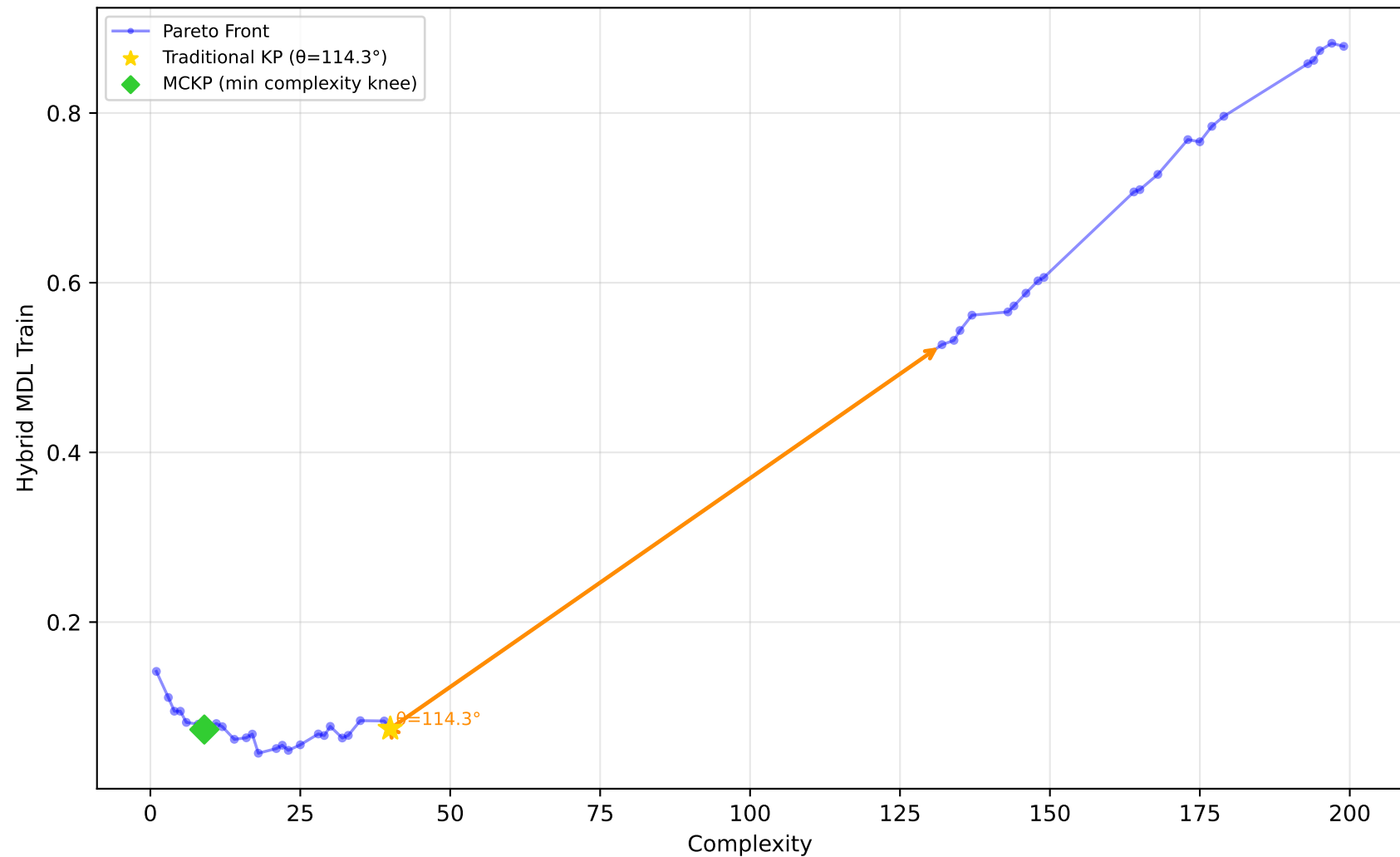
605_fri_c2_250_25 - Run 18 - SVP - Hybrid MDL Train \lambda_1=0.10, \bar{\lambda}_2=0.00, \bar{\lambda}_3=0.00 | Difficulty: 1.00 | Method: hmr
