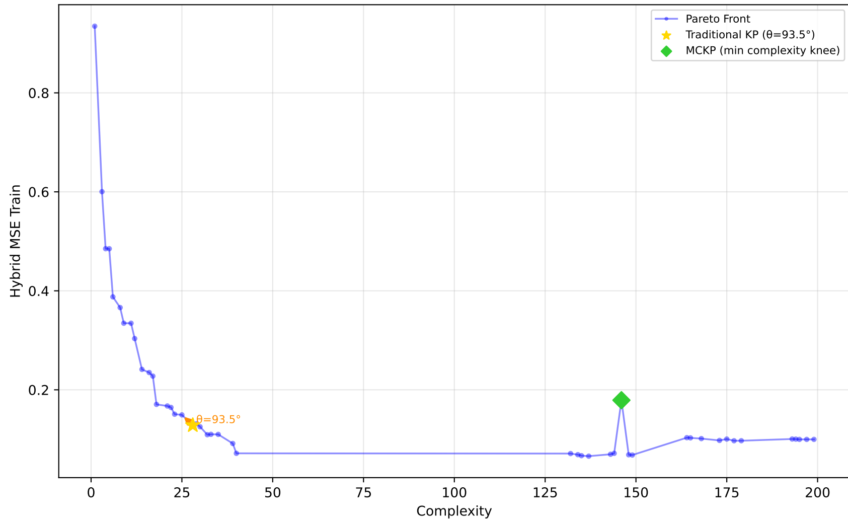
605_fri_c2_250_25 - Run 18 - SVP - Hybrid MSE Train \lambda_1=0.40, \lambda_2=0.00, \lambda_3=0.20 | Difficulty: 1.00 | Method: hmr
