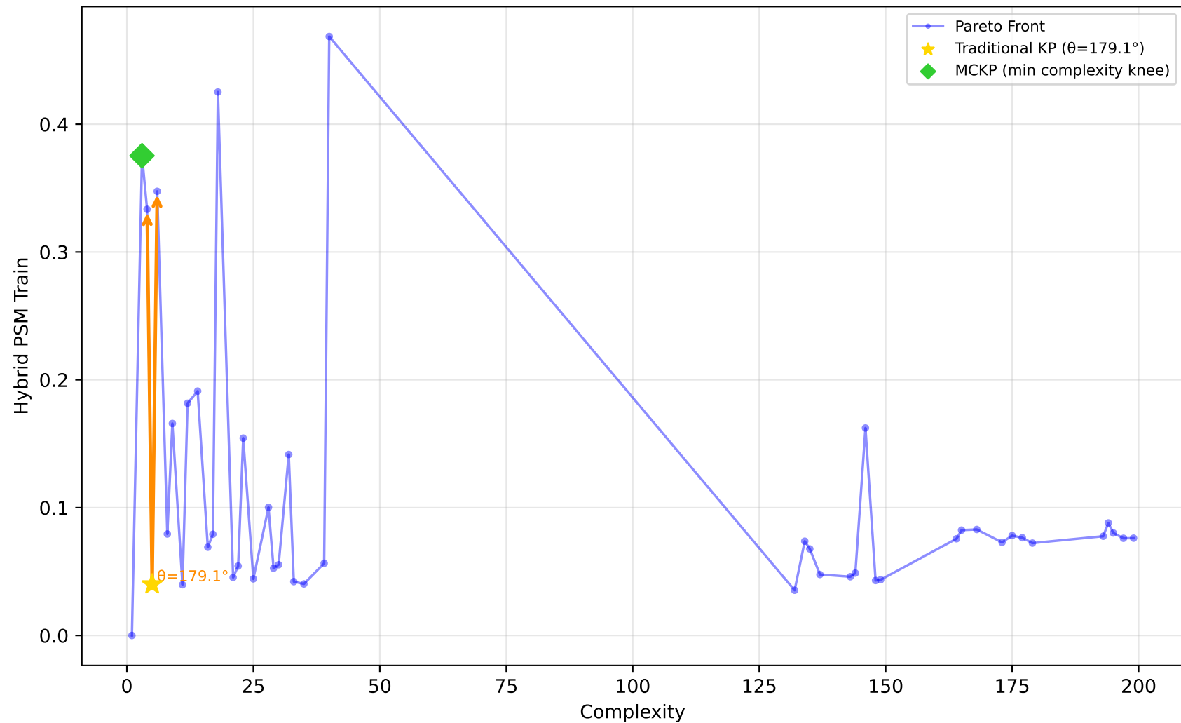
605_fri_c2_250_25 - Run 18 - SVP - Hybrid PSM Train \lambda_1=0.40, \lambda_2=0.00, \lambda_3=0.20 | Difficulty: 1.00 | Method: hmr
