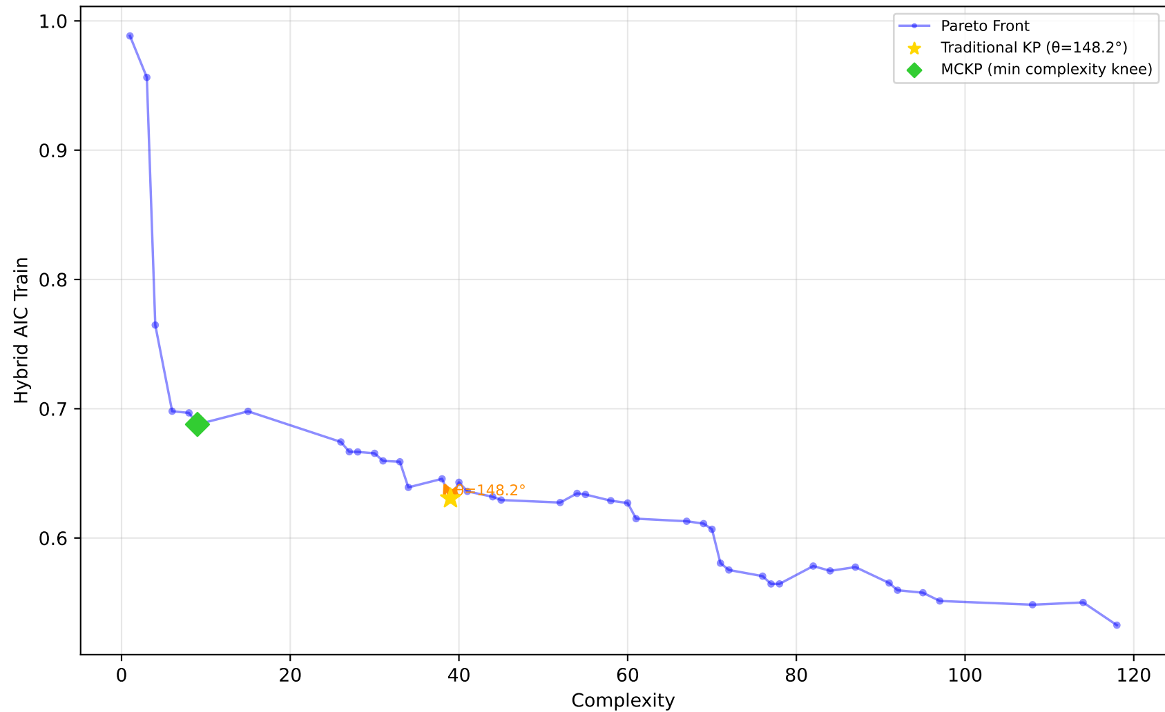
605_fri_c2_250_25 - Run 19 - MVP - Hybrid AIC Train \lambda_1=0.30, \lambda_2=0.00, \lambda_3=1.00 | Difficulty: 1.00 | Method: hmr
