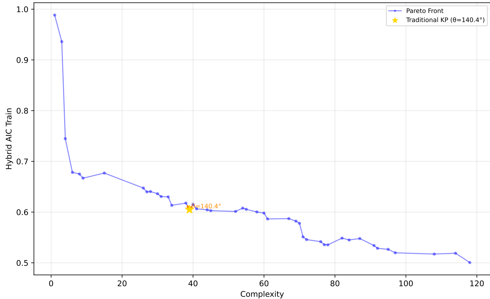
605_fri_c2_250_25 - Run 19 - SVP - Hybrid AIC Train \lambda_1=0.10, \lambda_2=0.00, \lambda_3=0.00 | Difficulty: 1.00 | Method: hmr
