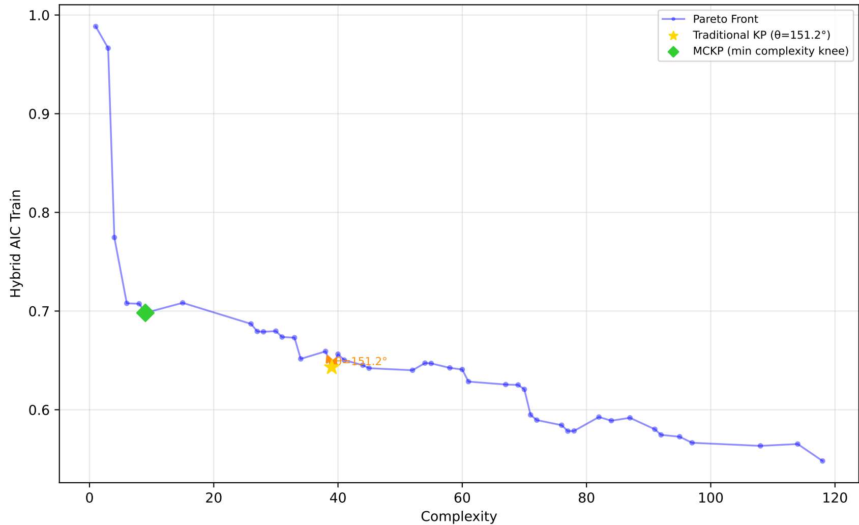
605_fri_c2_250_25 - Run 19 - SVP - Hybrid AIC Train \lambda_1=0.40 , \lambda_2=0.00 , \lambda_3=0.20 | Difficulty: 1.00 | Method: hmr
