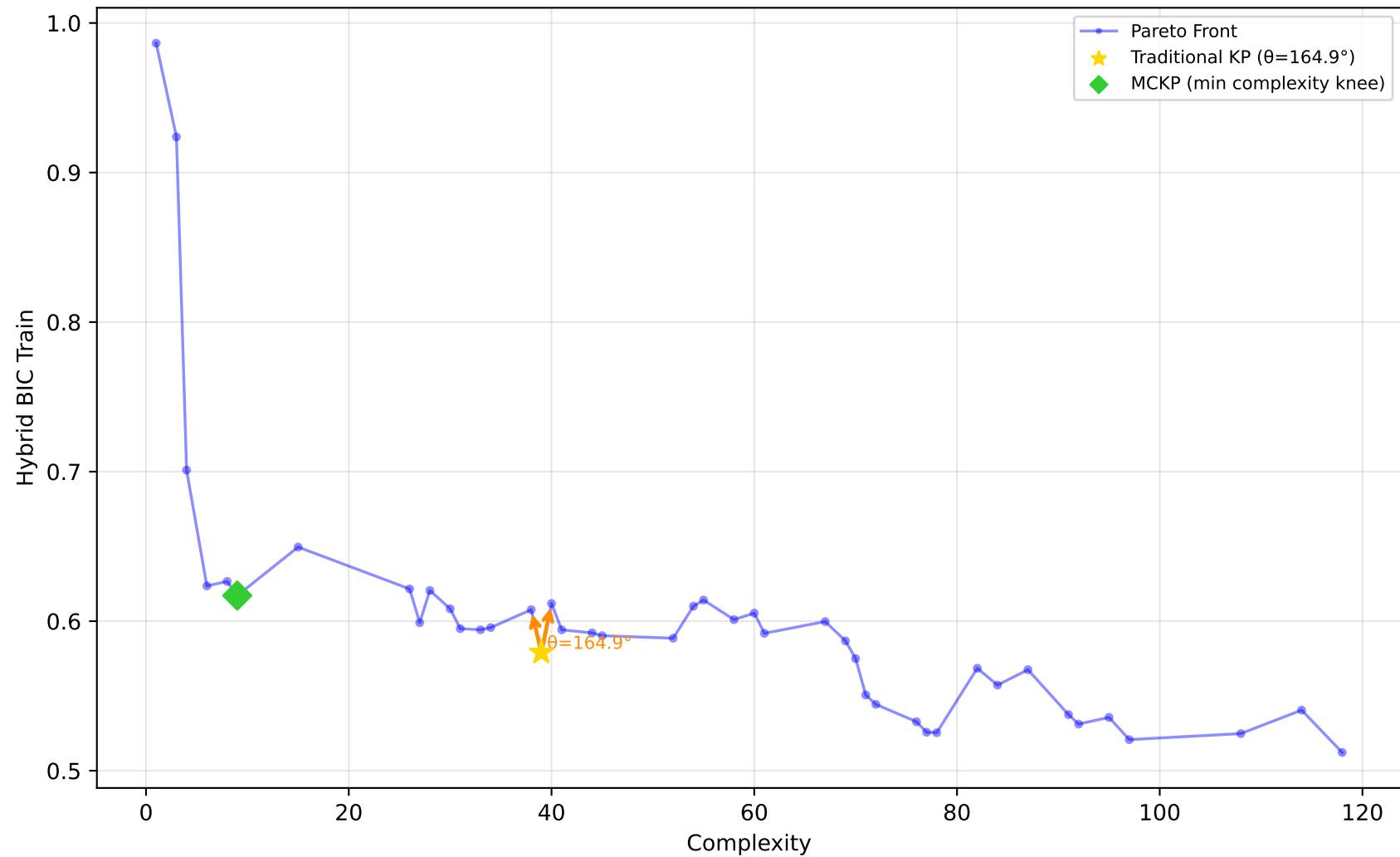
605_fri_c2_250_25 - Run 19 - SVP - Hybrid BIC Train \lambda_1=0.10, \lambda_2=0.00, \lambda_3=0.00 | Difficulty: 1.00 | Method: hmr
