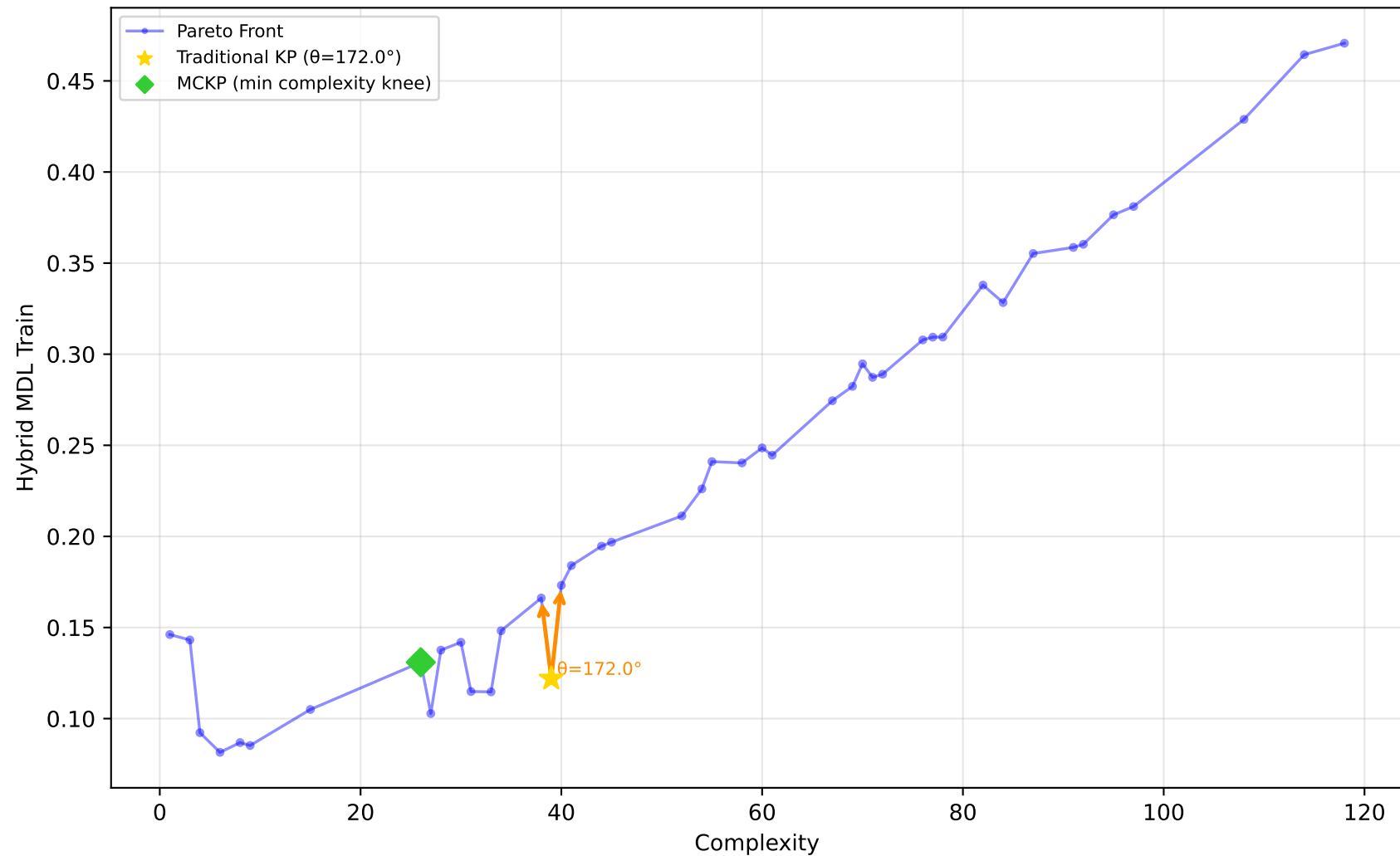
605_fri_c2_250_25 - Run 19 - SVP - Hybrid MDL Train \lambda_1=0.10, \lambda_2=0.00, \lambda_3=0.00 | Difficulty: 1.00 | Method: hmr
