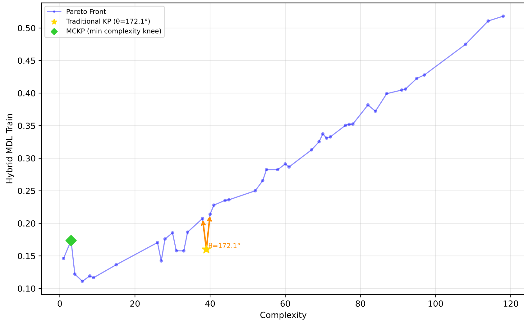
605_fri_c2_250_25 - Run 19 - SVP - Hybrid MDL Train \lambda_1=0.40 , \lambda_2=0.00 , \lambda_3=0.20 | Difficulty: 1.00 | Method: hmr
