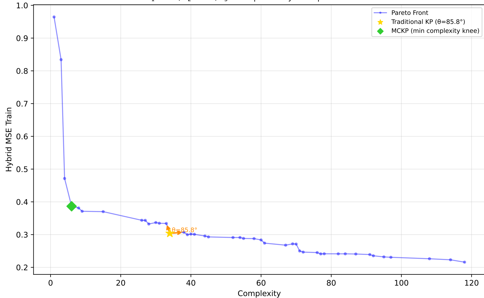
605_fri_c2_250_25 - Run 19 - SVP - Hybrid MSE Train \lambda_1=0.40, \lambda_2=0.00, \lambda_3=0.20 | Difficulty: 1.00 | Method: hmr
