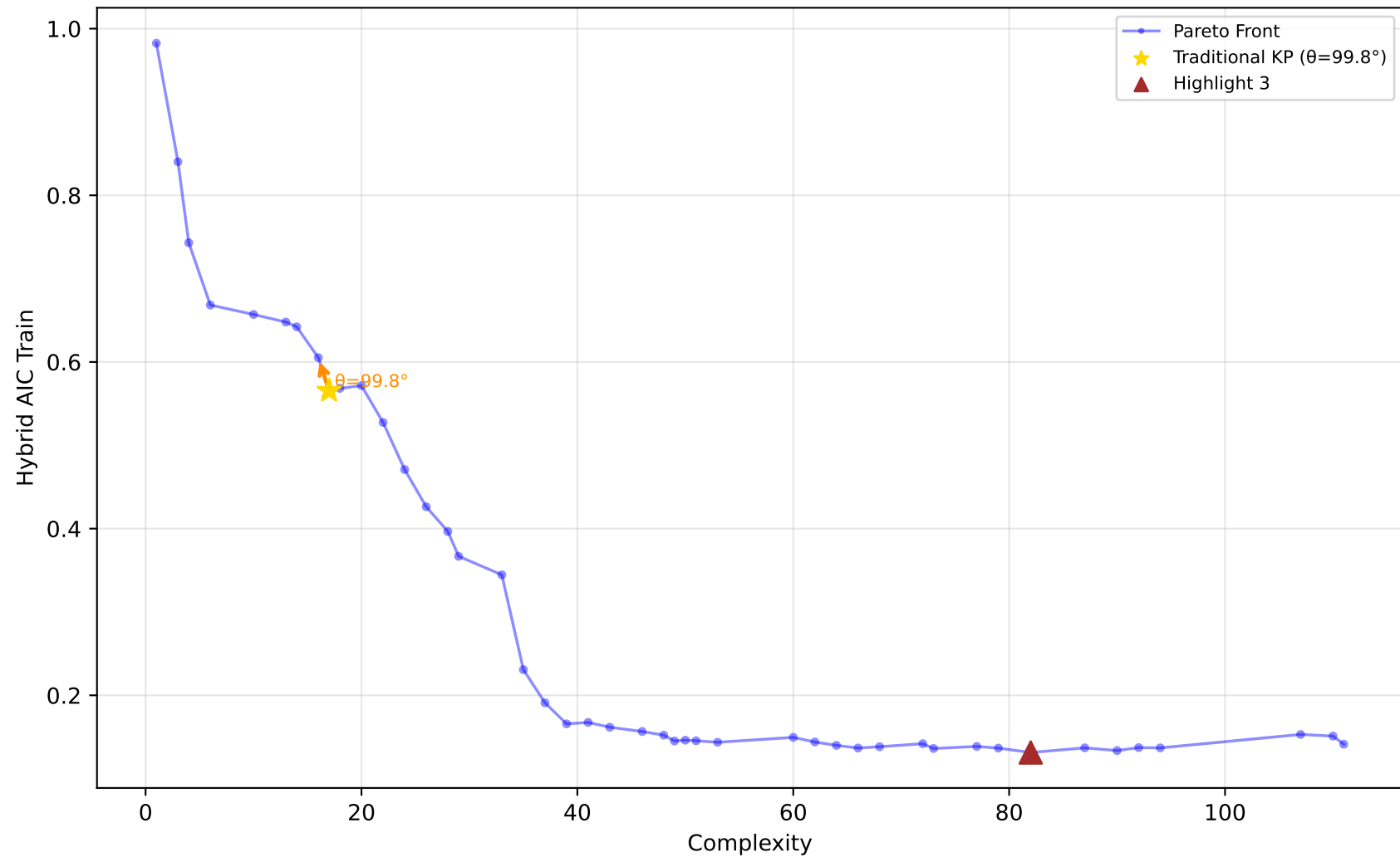
605_fri_c2_250_25 - Run 1 - MVP - Hybrid AIC Train \lambda_1=0.10, \lambda_2=0.00, \lambda_3=0.00 | Difficulty: 1.00 | Method: hmr
