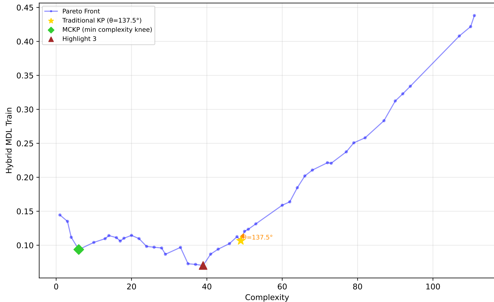
605_fri_c2_250_25 - Run 1 - MVP - Hybrid MDL Train \lambda_1=0.30 , \lambda_2=0.00 , \lambda_3=1.00 | Difficulty: 1.00 | Method: hmr
