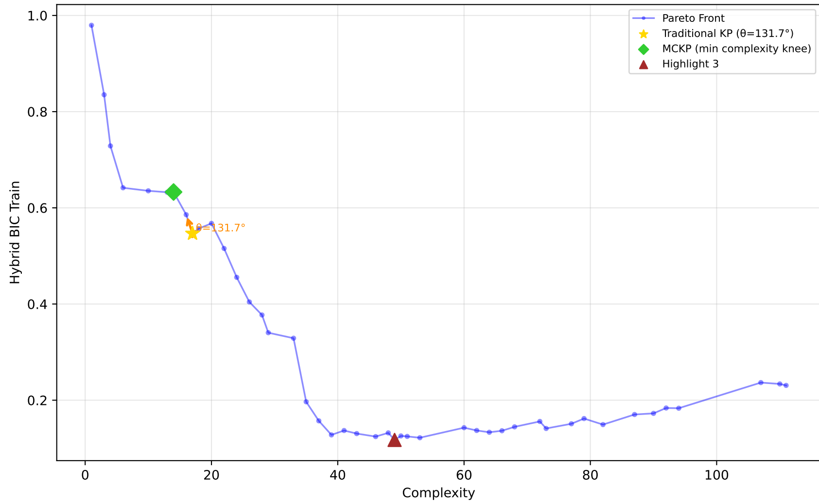
605_fri_c2_250_25 - Run 1 - SVP - Hybrid BIC Train \lambda_1=0.40, \lambda_2=0.00, \lambda_3=0.20 | Difficulty: 1.00 | Method: hmr
