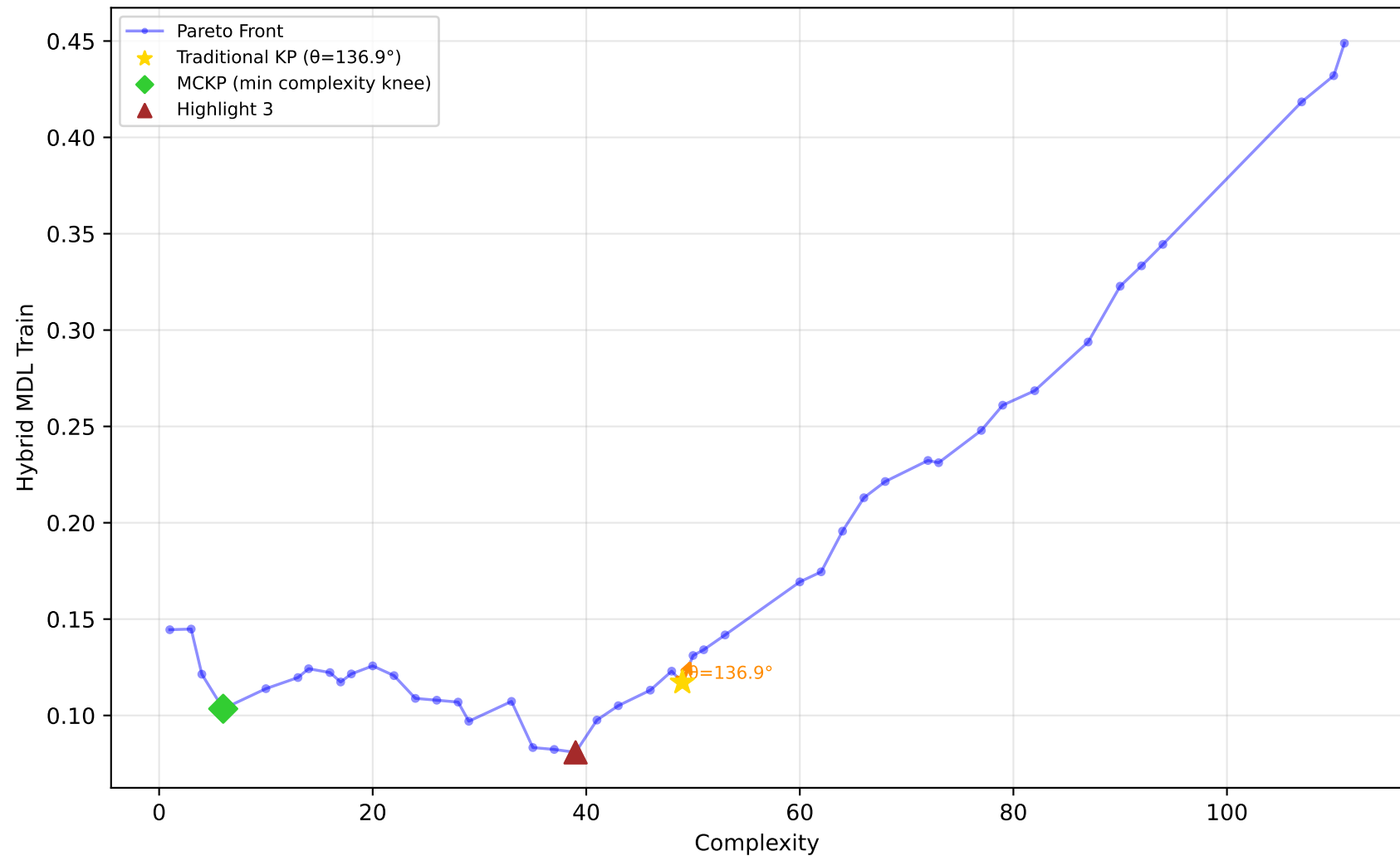
605_fri_c2_250_25 - Run 1 - SVP - Hybrid MDL Train \lambda_1=0.40, \lambda_2=0.00, \bar{\lambda}_3=0.20 | Difficulty: 1.00 | Method: hmr
