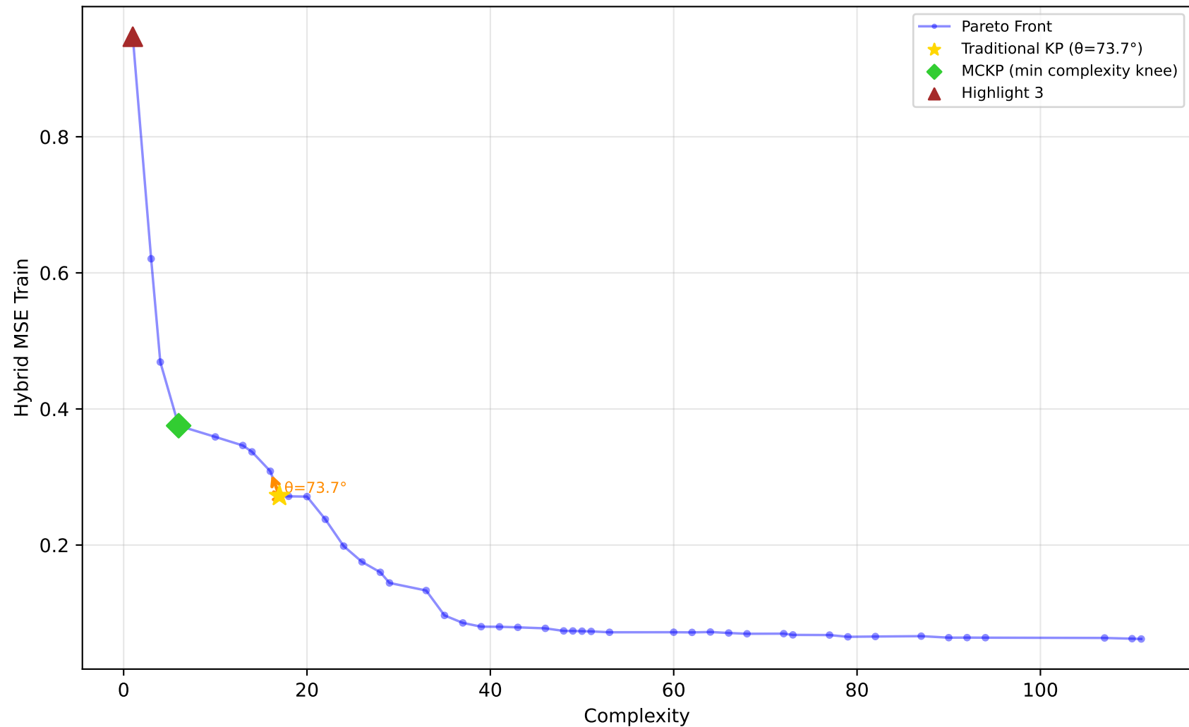
605_fri_c2_250_25 - Run 1 - SVP - Hybrid MSE Train \lambda_1=0.40, \lambda_2=0.00, \lambda_3=0.20 | Difficulty: 1.00 | Method: hmr
