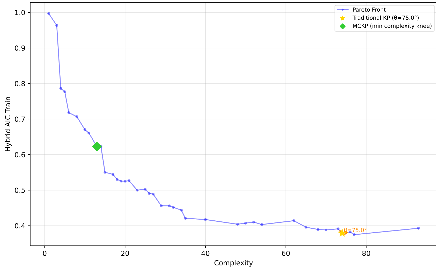
605_fri_c2_250_25 - Run 20 - MVP - Hybrid AIC Train \lambda_1=0.30, \lambda_2=0.00, \lambda_3=1.00 | Difficulty: 1.00 | Method: hmr
