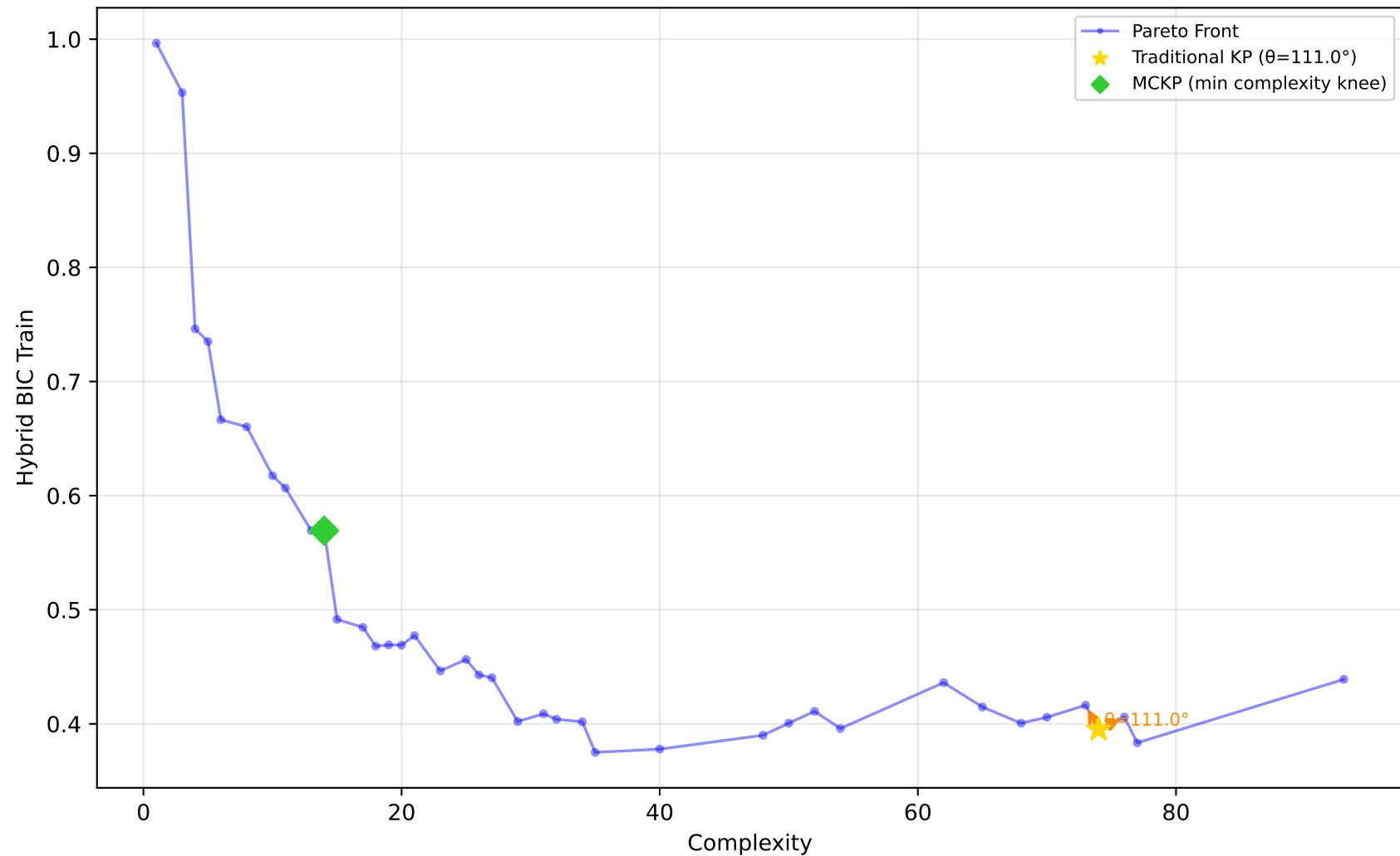
605_fri_c2_250_25 - Run 20 - MVP - Hybrid BIC Train \lambda_1=0.30, \lambda_2=0.00, \lambda_3=1.00 | Difficulty: 1.00 | Method: hmr
