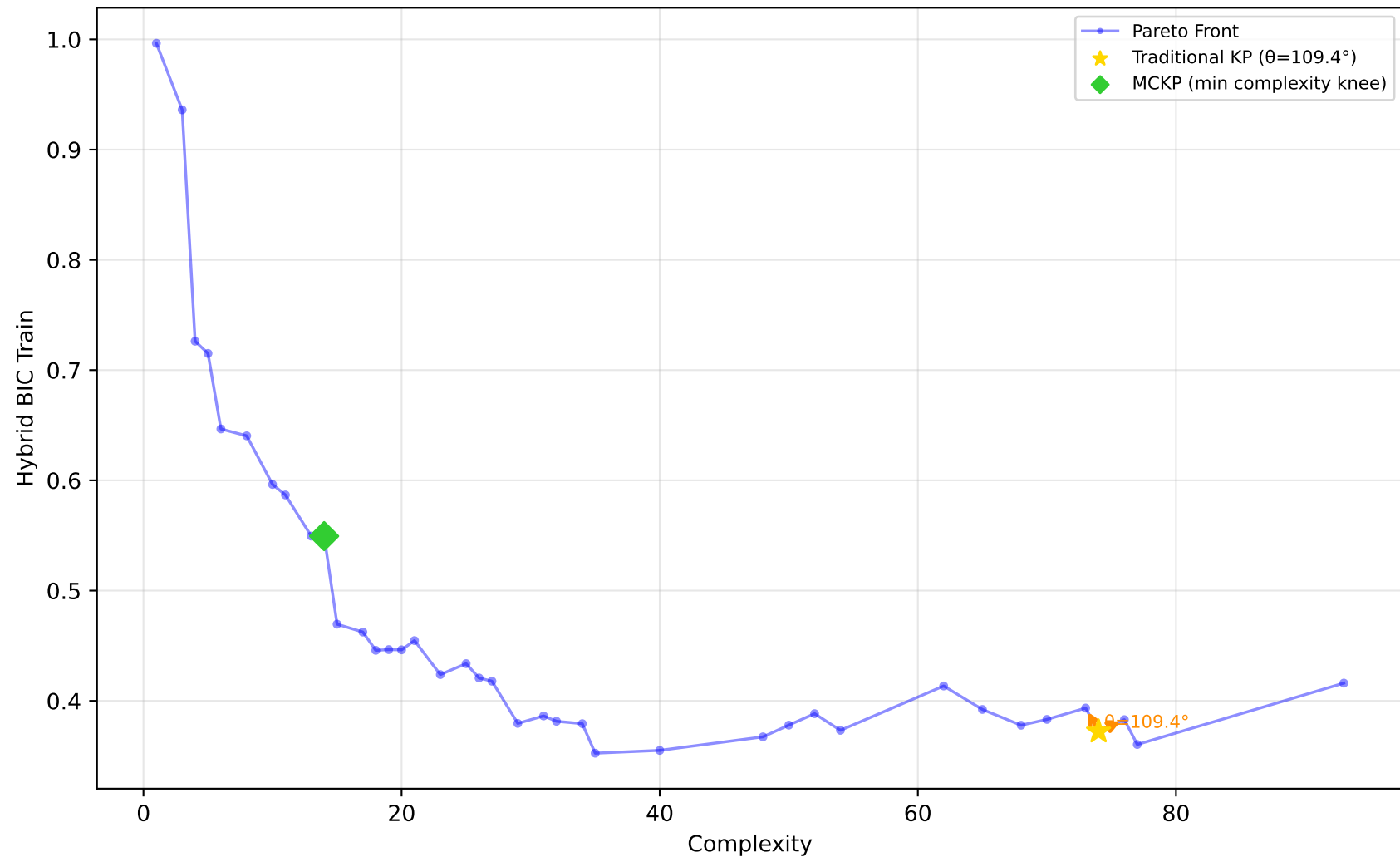
605_fri_c2_250_25 - Run 20 - SVP - Hybrid BIC Train \lambda_1=0.10, \lambda_2=0.00, \lambda_3=0.00 | Difficulty: 1.00 | Method: hmr
