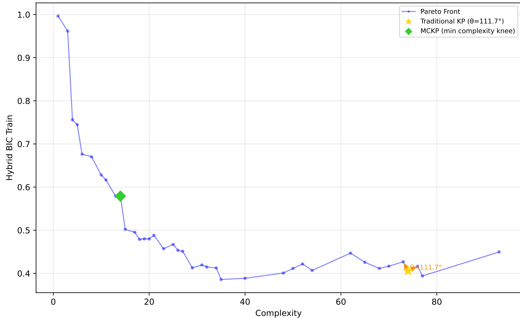
605_fri_c2_250_25 - Run 20 - SVP - Hybrid BIC Train \lambda_1=0.40, \lambda_2=0.00, \lambda_3=0.20 | Difficulty: 1.00 | Method: hmr
