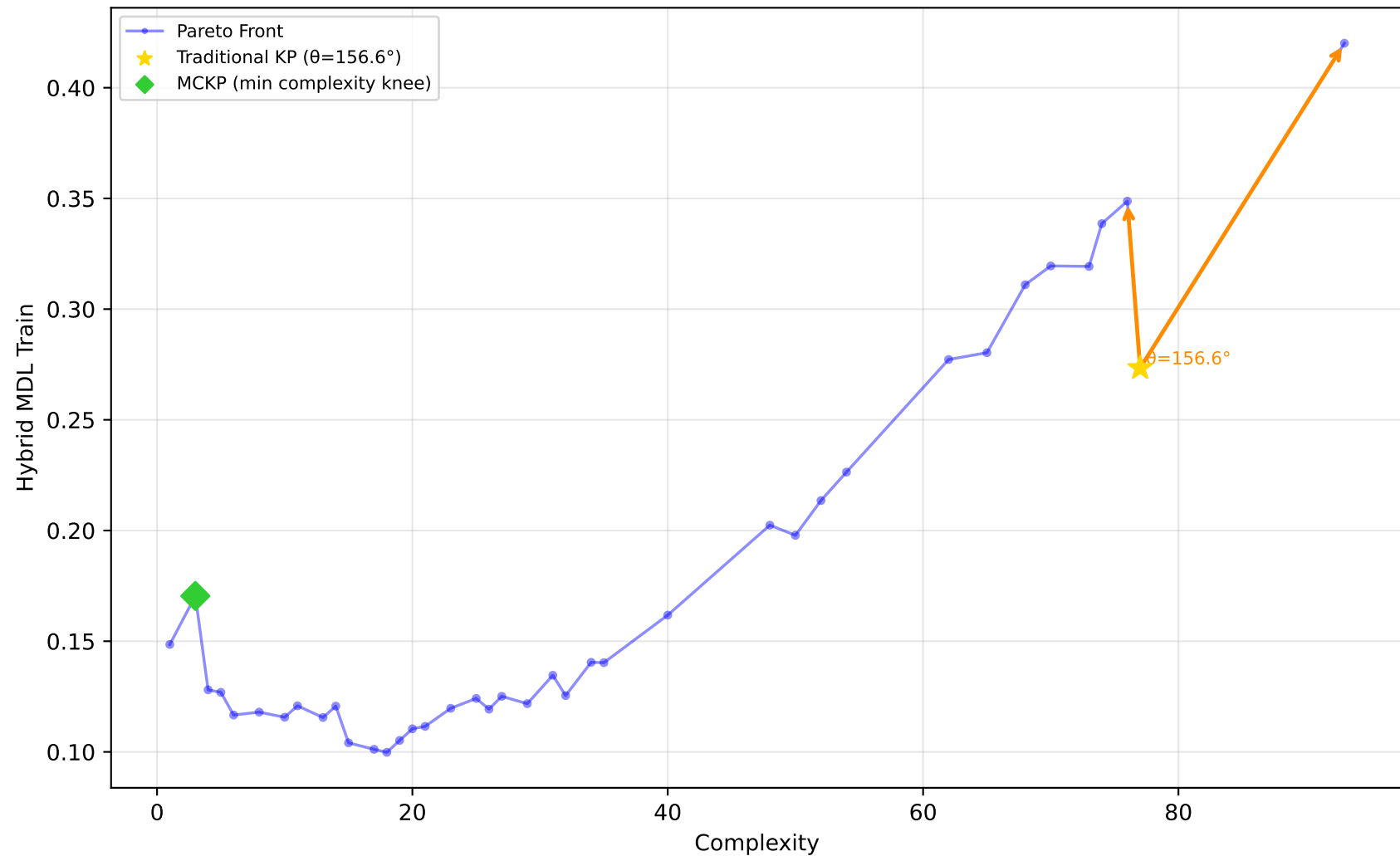
605_fri_c2_250_25 - Run 20 - SVP - Hybrid MDL Train \lambda_1=0.40, \lambda_2=0.00, \lambda_3=0.20 | Difficulty: 1.00 | Method: hmr
