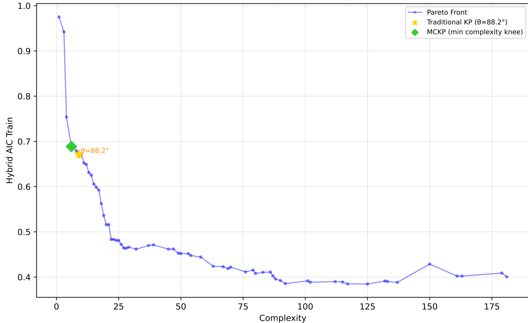
605_fri_c2_250_25 - Run 21 - MVP - Hybrid AIC Train \lambda_1=0.30, \lambda_2=0.00, \lambda_3=1.00 | Difficulty: 1.00 | Method: hmr
