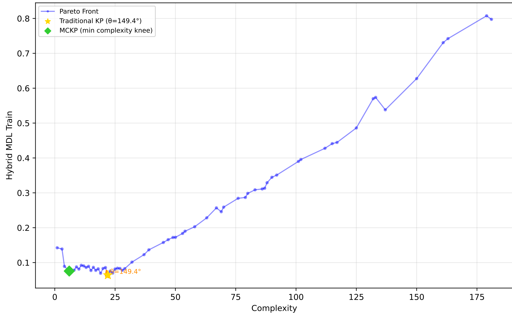
605_fri_c2_250_25 - Run 21 - MVP - Hybrid MDL Train \lambda_1=0.10, \bar{\lambda}_2=0.00, \bar{\lambda}_3=0.00 | Difficulty: 1.00 | Method: hmr
