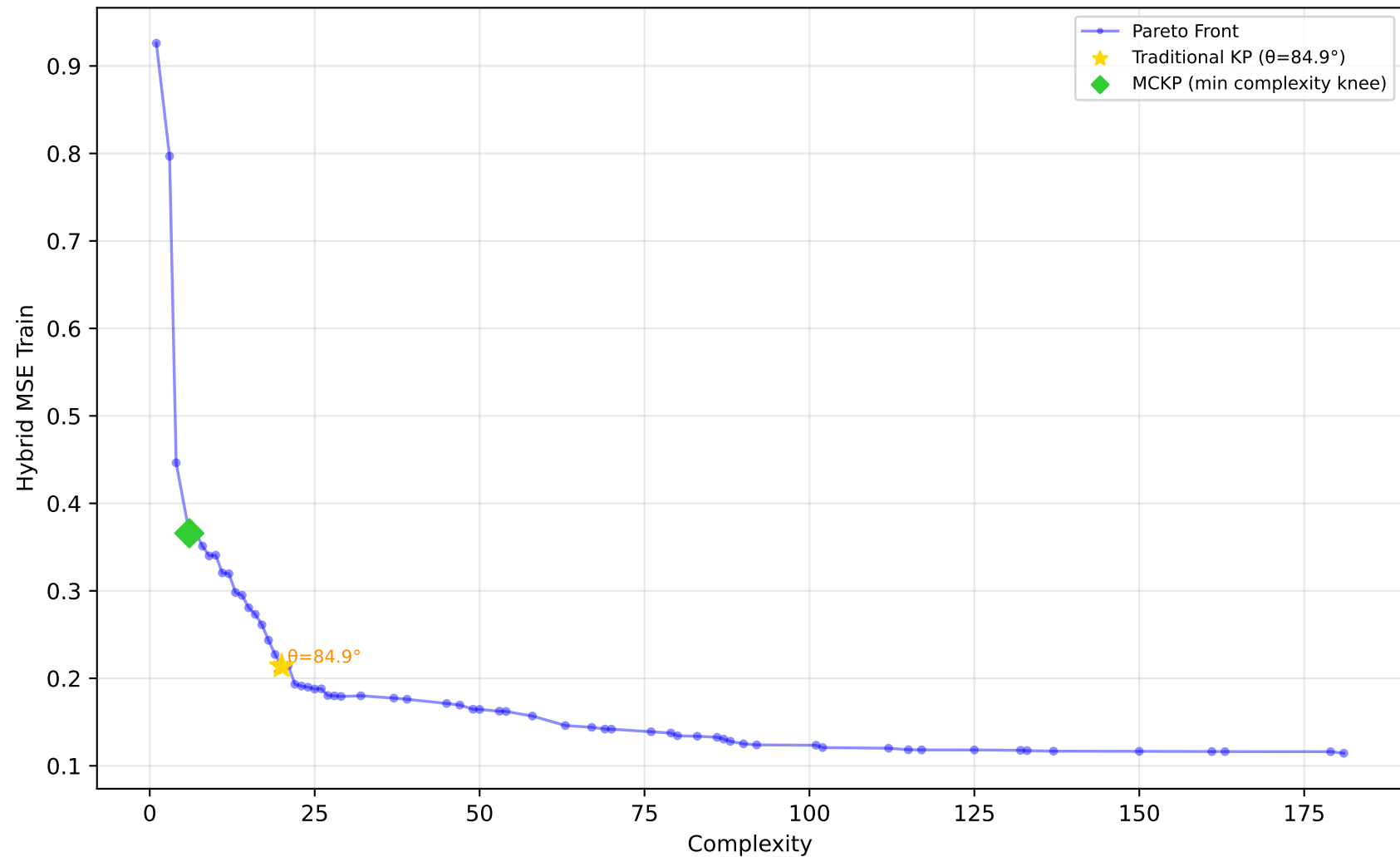
605_fri_c2_250_25 - Run 21 - MVP - Hybrid MSE Train \lambda_1=0.30, \bar{\lambda}_2=0.00, \bar{\lambda}_3=1.00 | Difficulty: 1.00 | Method: hmr
