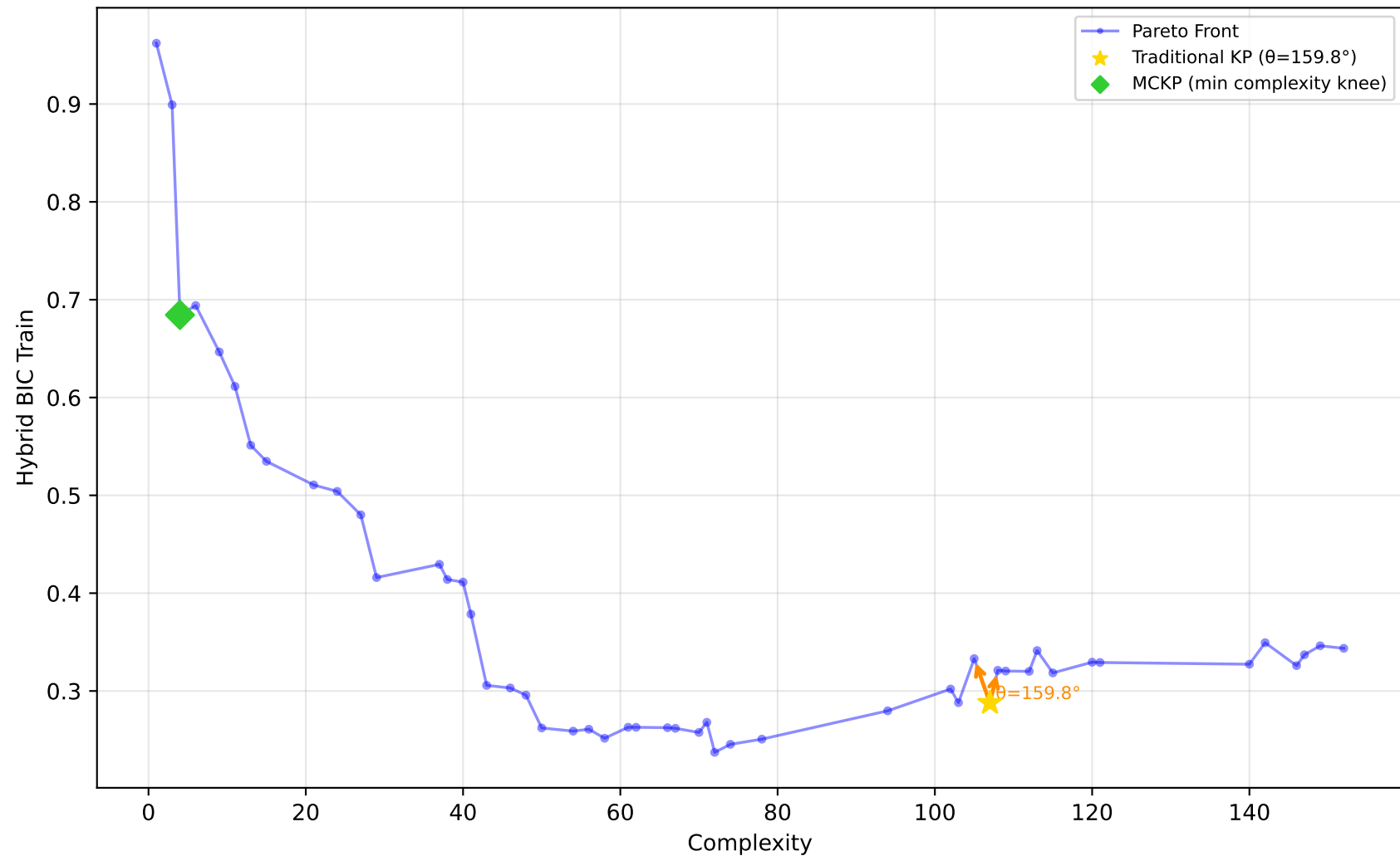
605_fri_c2_250_25 - Run 22 - MVP - Hybrid BIC Train \lambda_1=0.10, \lambda_2=0.00, \lambda_3=0.00 | Difficulty: 1.00 | Method: hmr
